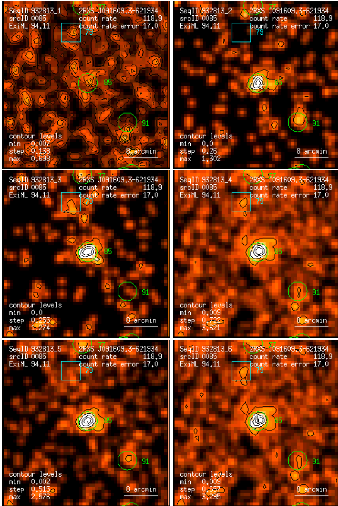
Figure 85: RASS 932813: detection 0085: band rate images, Gaussian filter: (1) PSPC channels 11 – 41, (2) 52 – 90, (3) 91 – 201, (4) 11 – 235, (5) 52 – 201, (6) 11 – 201. Broad band rates in counts/ks. Band rate contour levels in counts/ks/arcmin 2 .
