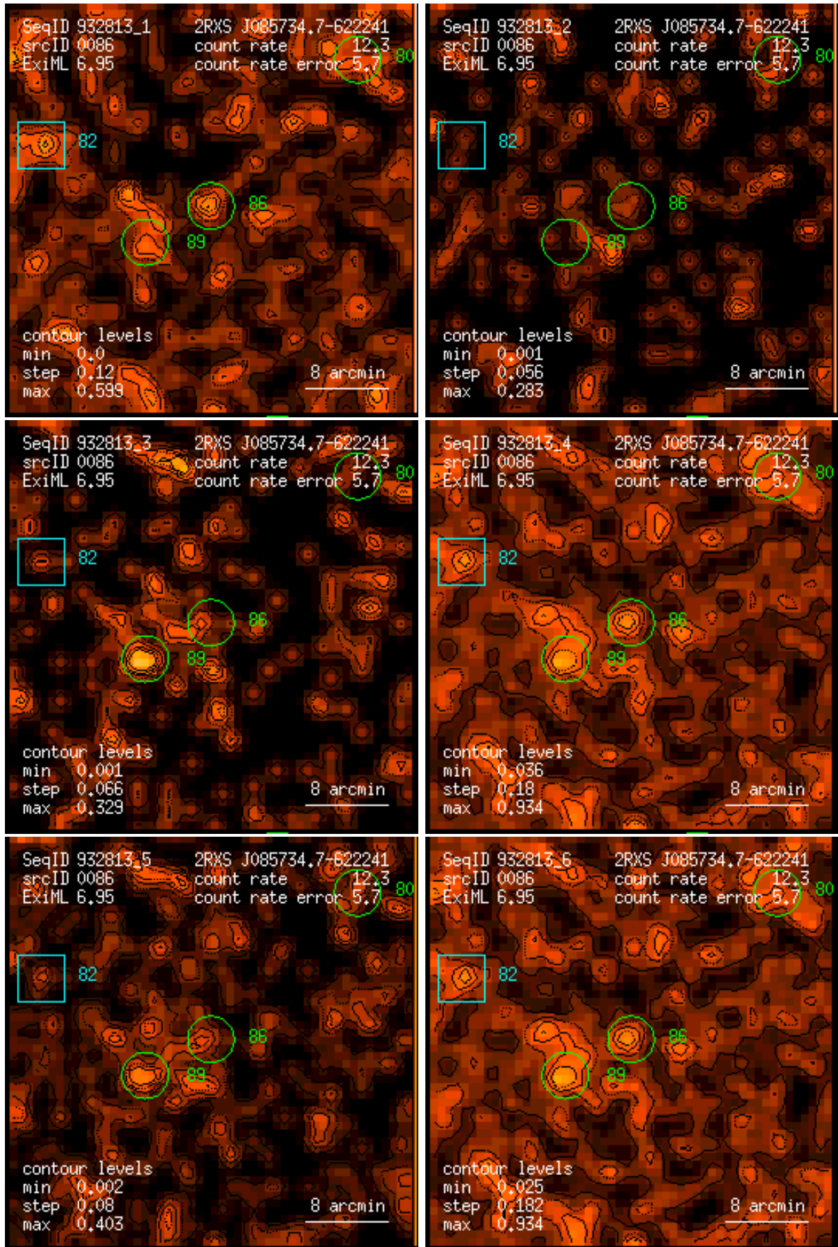
Figure 86: RASS 932813: detection 0086: band rate images, Gaussian filter: (1) PSPC channels 11 – 41, (2) 52 – 90, (3) 91 – 201, (4) 11 – 235, (5) 52 – 201, (6) 11 – 201. Broad band rates in counts/ks. Band rate contour levels in counts/ks/arcmin 2 .
