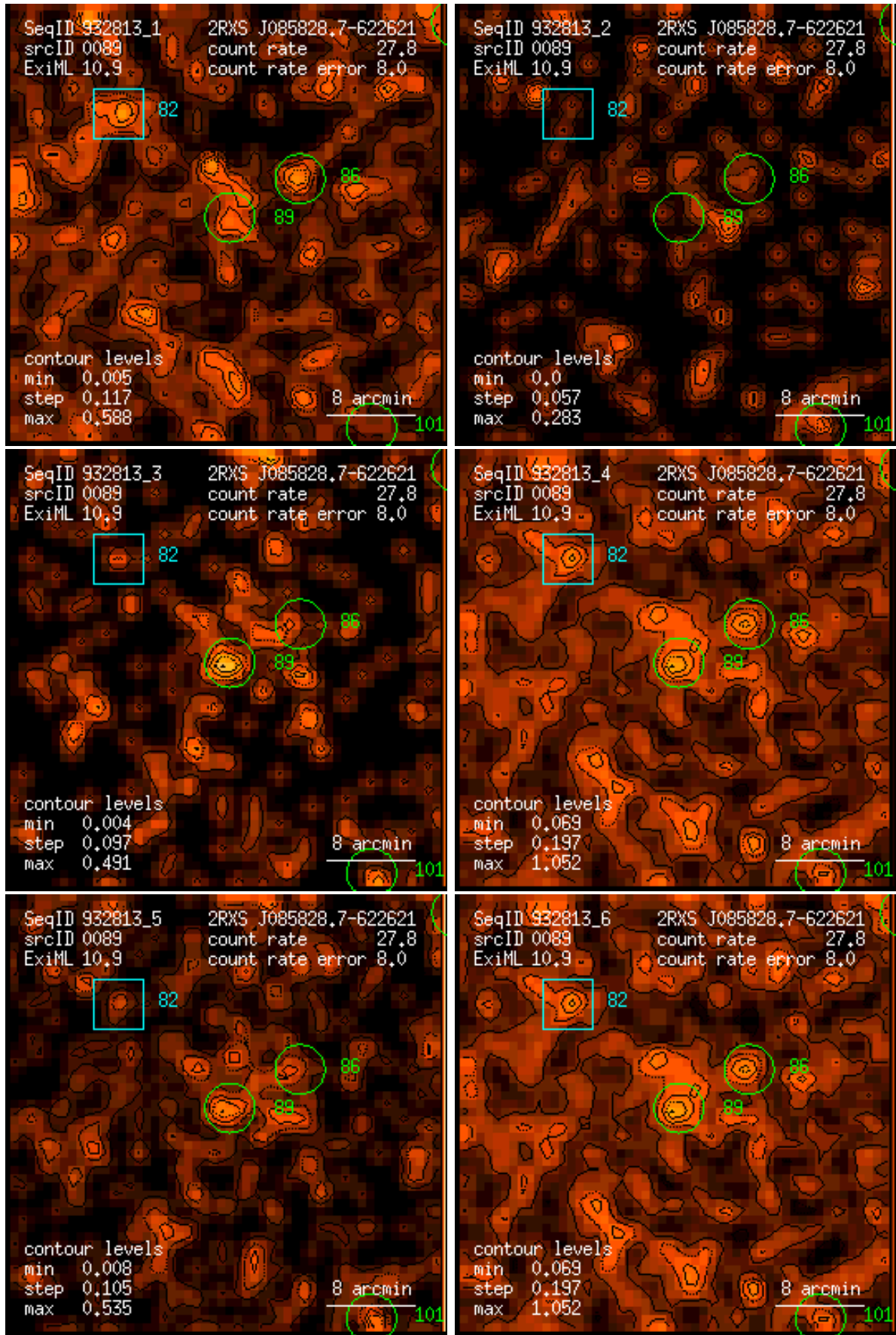
Figure 89: RASS 932813: detection 0089: band rate images, Gaussian filter: (1) PSPC channels 11 – 41, (2) 52 – 90, (3) 91 – 201, (4) 11 – 235, (5) 52 – 201, (6) 11 – 201. Broad band rates in counts/ks. Band rate contour levels in counts/ks/arcmin 2 .
