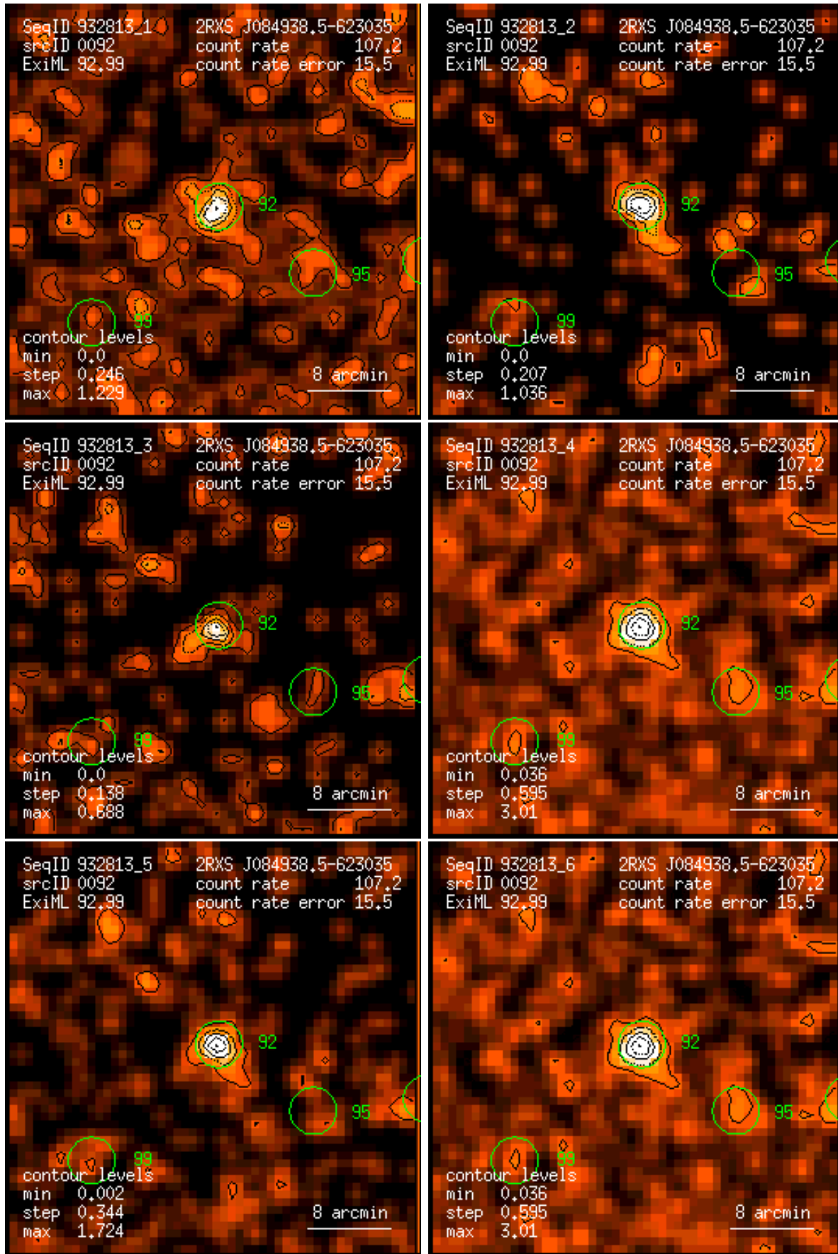
Figure 92: RASS 932813: detection 0092: band rate images, Gaussian filter: (1) PSPC channels 11 – 41, (2) 52 – 90, (3) 91 – 201, (4) 11 – 235, (5) 52 – 201, (6) 11 – 201. Broad band rates in counts/ks. Band rate contour levels in counts/ks/arcmin 2 .
