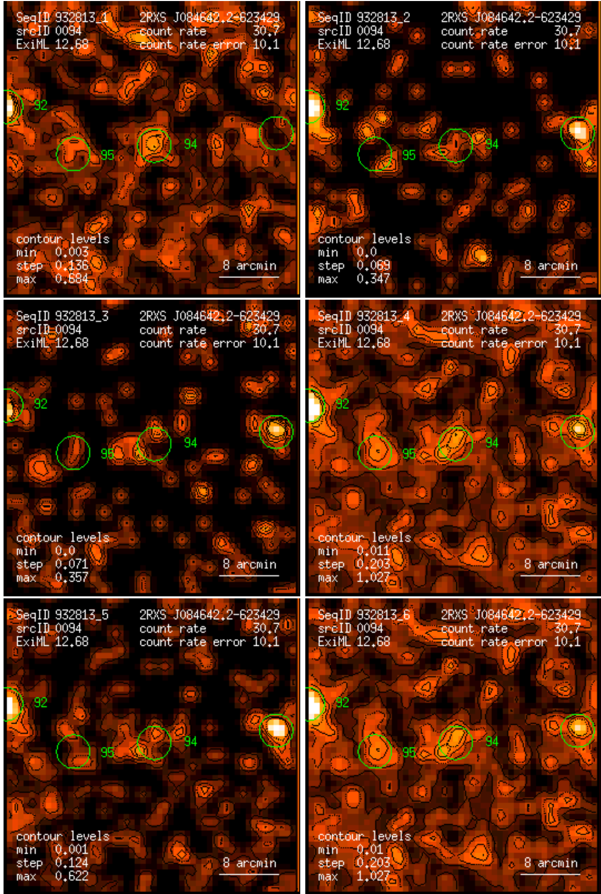
Figure 94: RASS 932813: detection 0094: band rate images, Gaussian filter: (1) PSPC channels 11 – 41, (2) 52 – 90, (3) 91 – 201, (4) 11 – 235, (5) 52 – 201, (6) 11 – 201. Broad band rates in counts/ks. Band rate contour levels in counts/ks/arcmin 2 .
