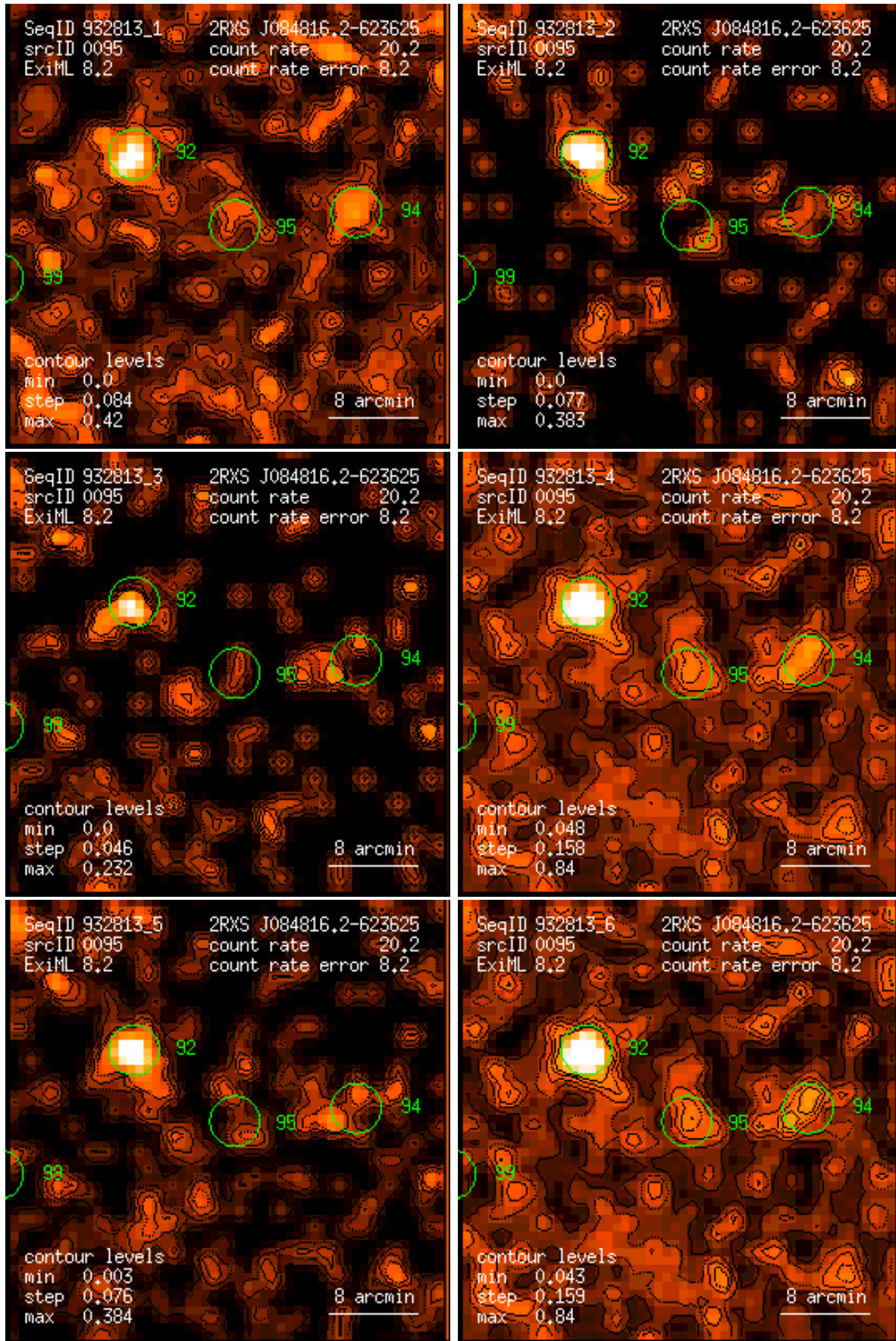
Figure 95: RASS 932813: detection 0095: band rate images, Gaussian filter: (1) PSPC channels 11 – 41, (2) 52 – 90, (3) 91 – 201, (4) 11 – 235, (5) 52 – 201, (6) 11 – 201. Broad band rates in counts/ks. Band rate contour levels in counts/ks/arcmin 2 .
