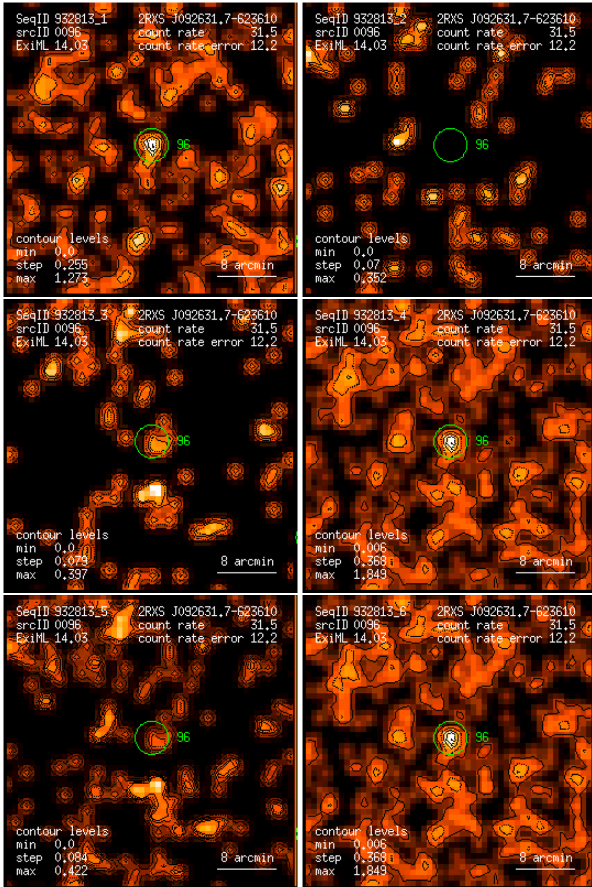
Figure 96: RASS 932813: detection 0096: band rate images, Gaussian filter: (1) PSPC channels 11 – 41, (2) 52 – 90, (3) 91 – 201, (4) 11 – 235, (5) 52 – 201, (6) 11 – 201. Broad band rates in counts/ks. Band rate contour levels in counts/ks/arcmin 2 .
