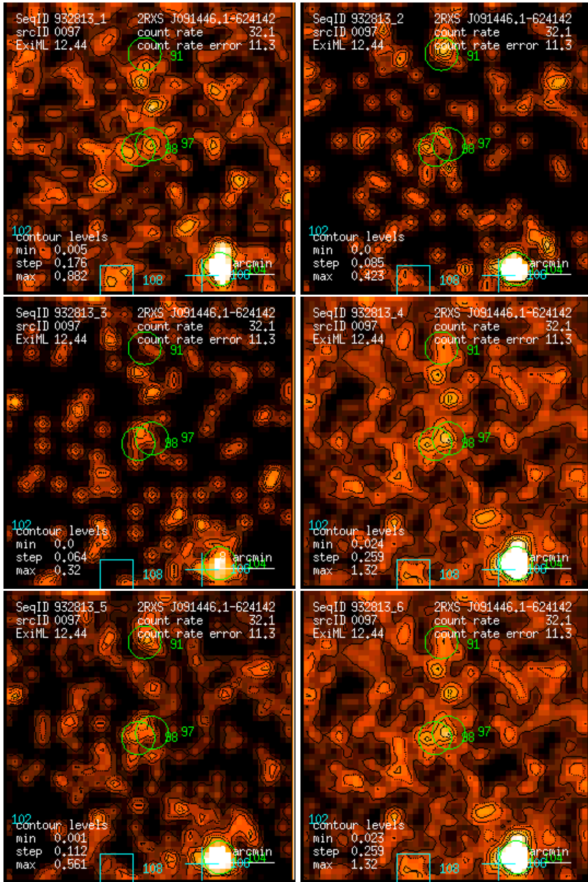
Figure 97: RASS 932813: detection 0097: band rate images, Gaussian filter: (1) PSPC channels 11 – 41, (2) 52 – 90, (3) 91 – 201, (4) 11 – 235, (5) 52 – 201, (6) 11 – 201. Broad band rates in counts/ks. Band rate contour levels in counts/ks/arcmin 2 .
