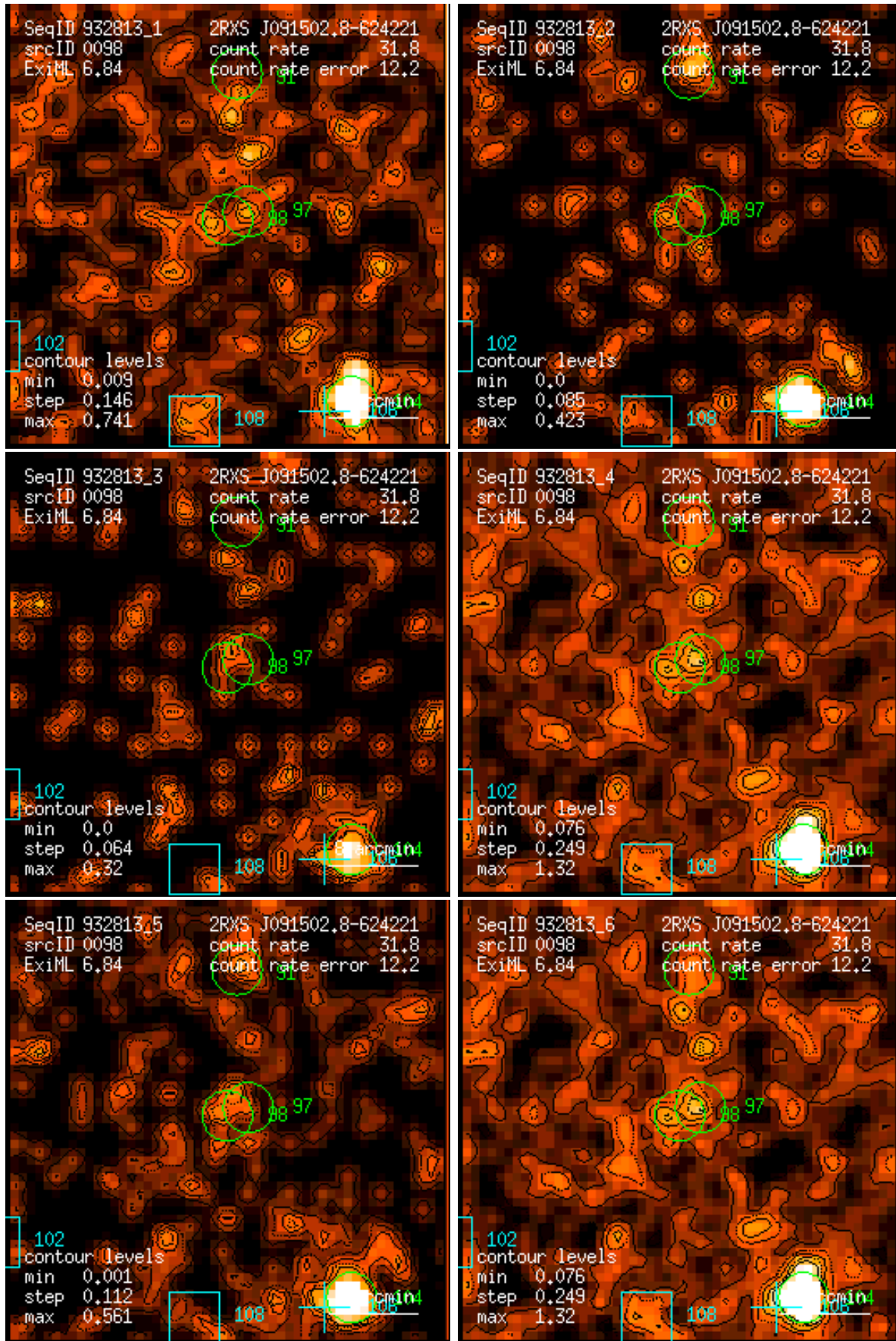
Figure 98: RASS 932813: detection 0098: band rate images, Gaussian filter: (1) PSPC channels 11 – 41, (2) 52 – 90, (3) 91 – 201, (4) 11 – 235, (5) 52 – 201, (6) 11 – 201. Broad band rates in counts/ks. Band rate contour levels in counts/ks/arcmin 2 .
