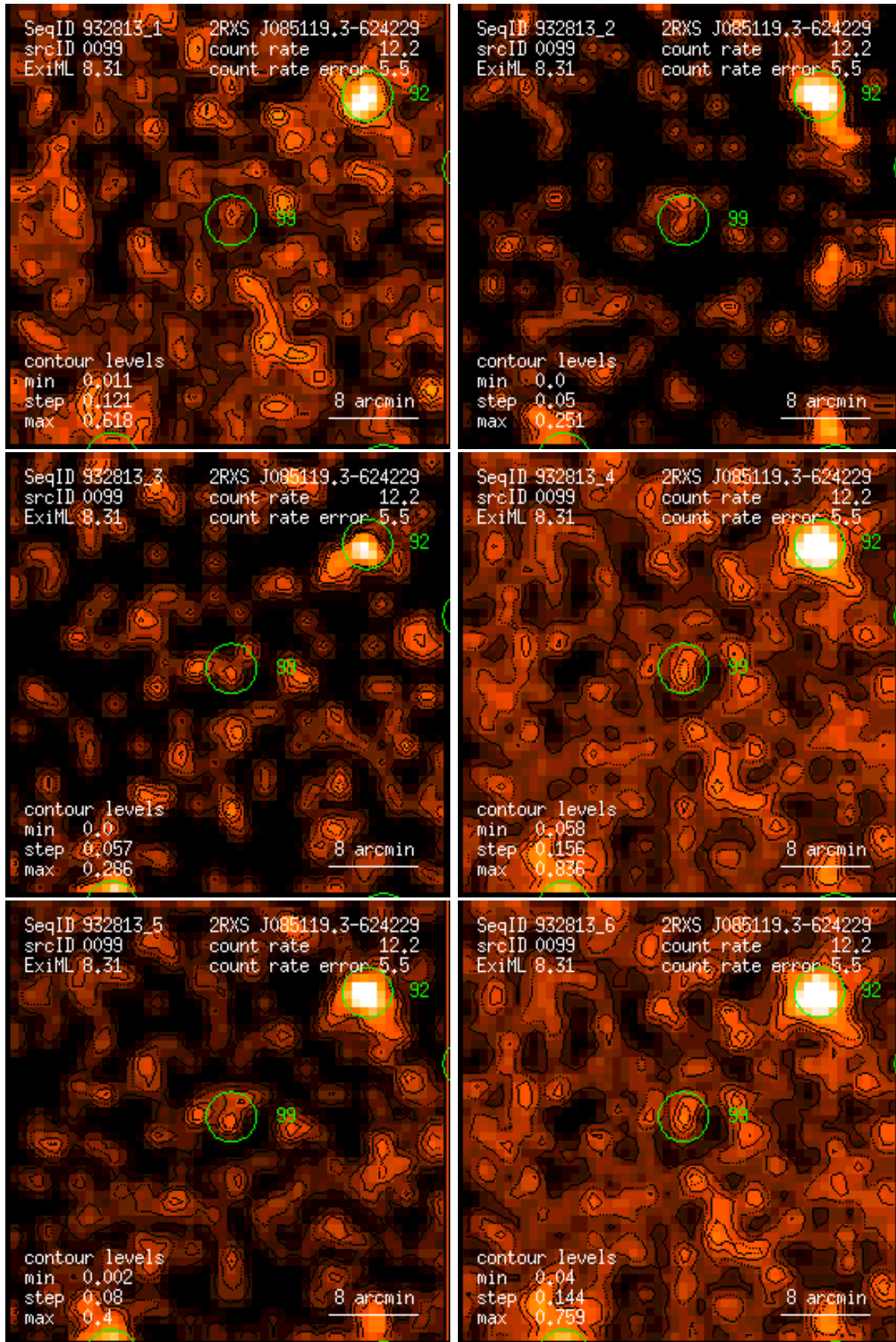
Figure 99: RASS 932813: detection 0099: band rate images, Gaussian filter: (1) PSPC channels 11 – 41, (2) 52 – 90, (3) 91 – 201, (4) 11 – 235, (5) 52 – 201, (6) 11 – 201. Broad band rates in counts/ks. Band rate contour levels in counts/ks/arcmin 2 .
