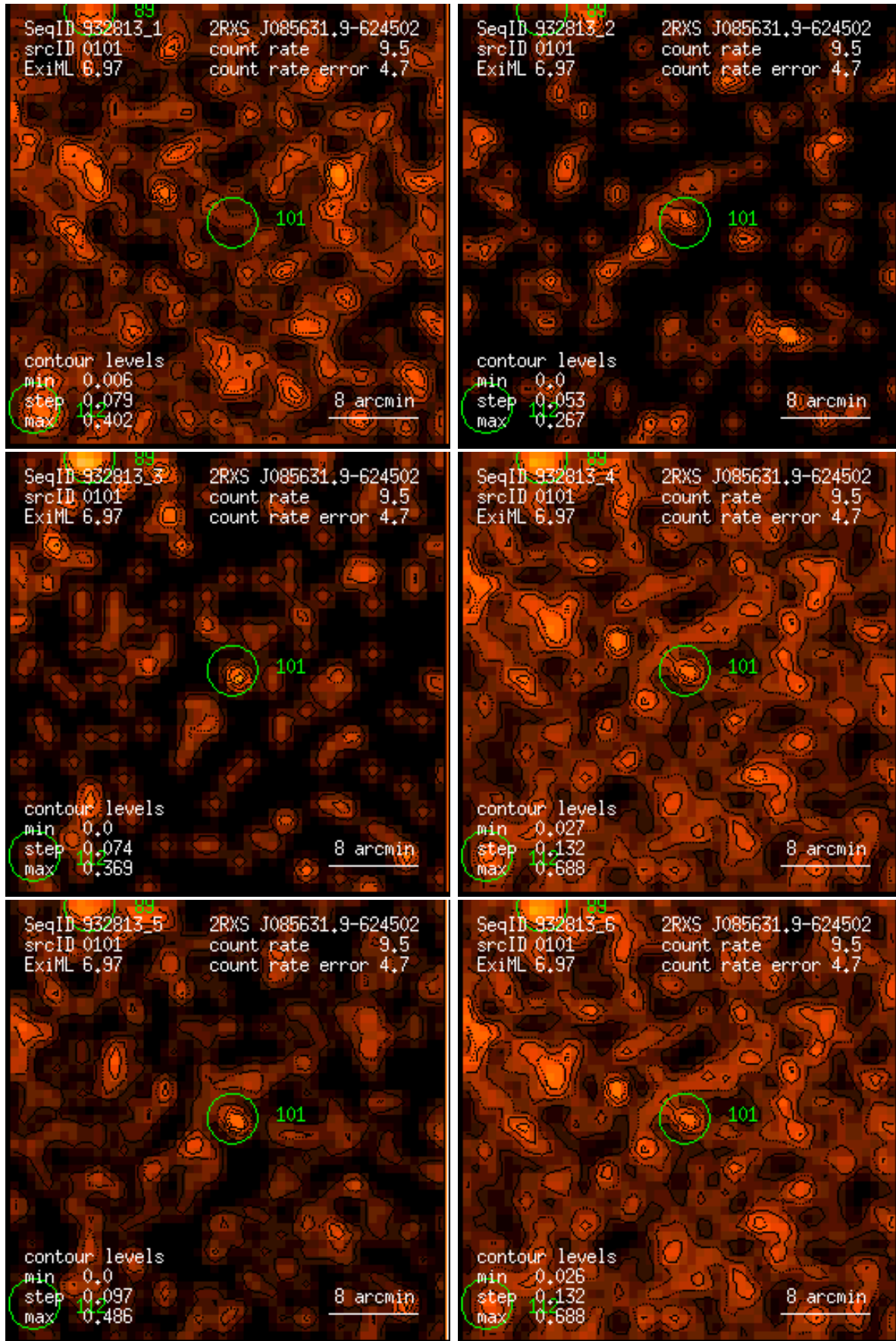
Figure 101: RASS 932813: detection 0101: band rate images, Gaussian filter: (1) PSPC channels 11 – 41, (2) 52 – 90, (3) 91 – 201, (4) 11 – 235, (5) 52 – 201, (6) 11 – 201. Broad band rates in counts/ks. Band rate contour levels in counts/ks/arcmin 2 .
