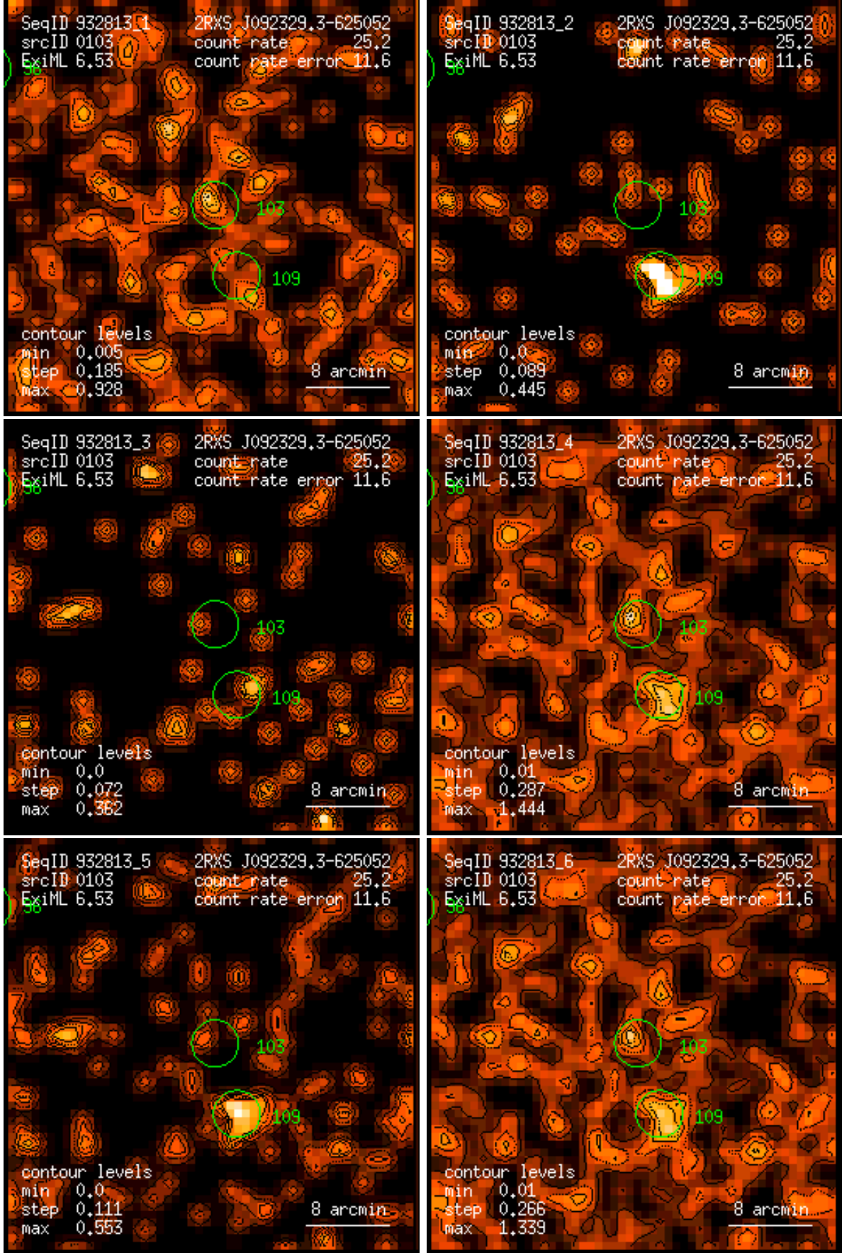
Figure 103: RASS 932813: detection 0103: band rate images, Gaussian filter: (1) PSPC channels 11 – 41, (2) 52 – 90, (3) 91 – 201, (4) 11 – 235, (5) 52 – 201, (6) 11 – 201. Broad band rates in counts/ks. Band rate contour levels in counts/ks/arcmin 2 .
