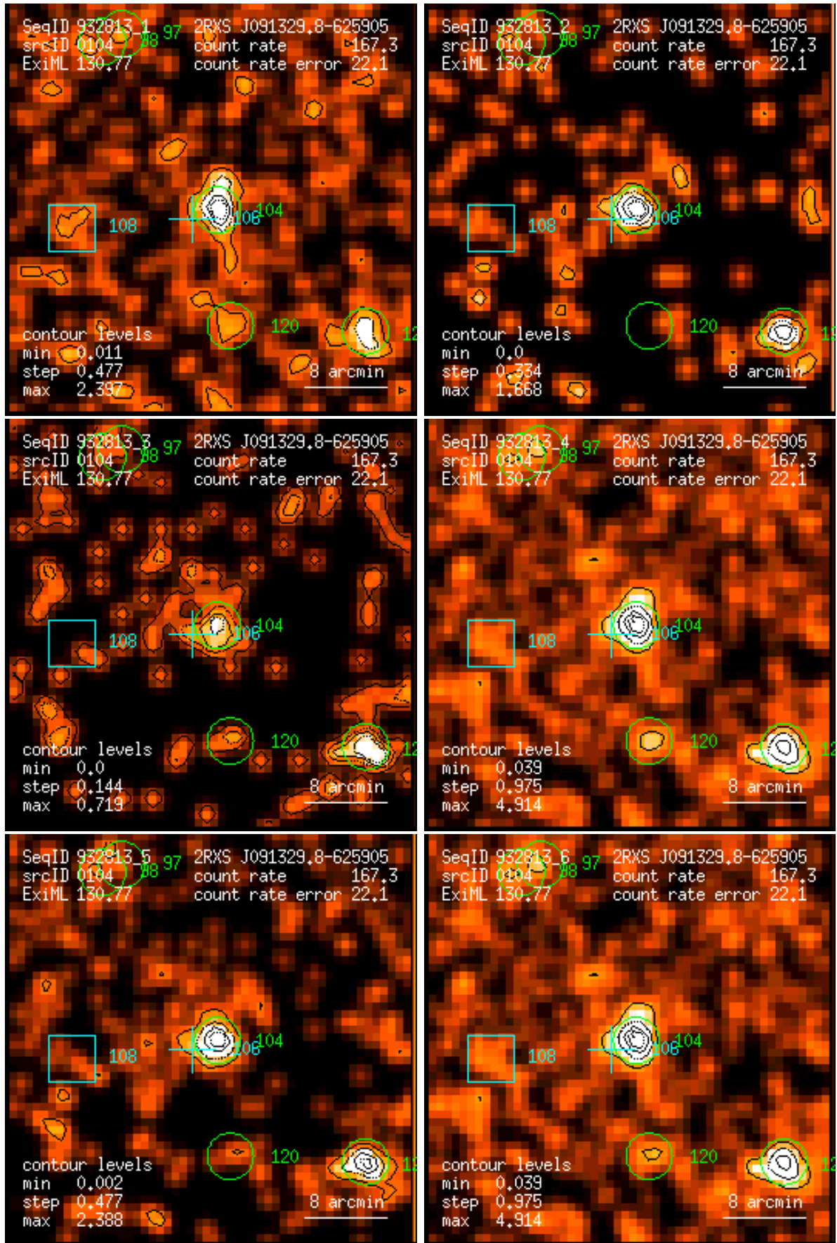
Figure 104: RASS 932813: detection 0104: band rate images, Gaussian filter: (1) PSPC channels 11 – 41, (2) 52 – 90, (3) 91 – 201, (4) 11 – 235, (5) 52 – 201, (6) 11 – 201. Broad band rates in counts/ks. Band rate contour levels in counts/ks/arcmin 2 .
