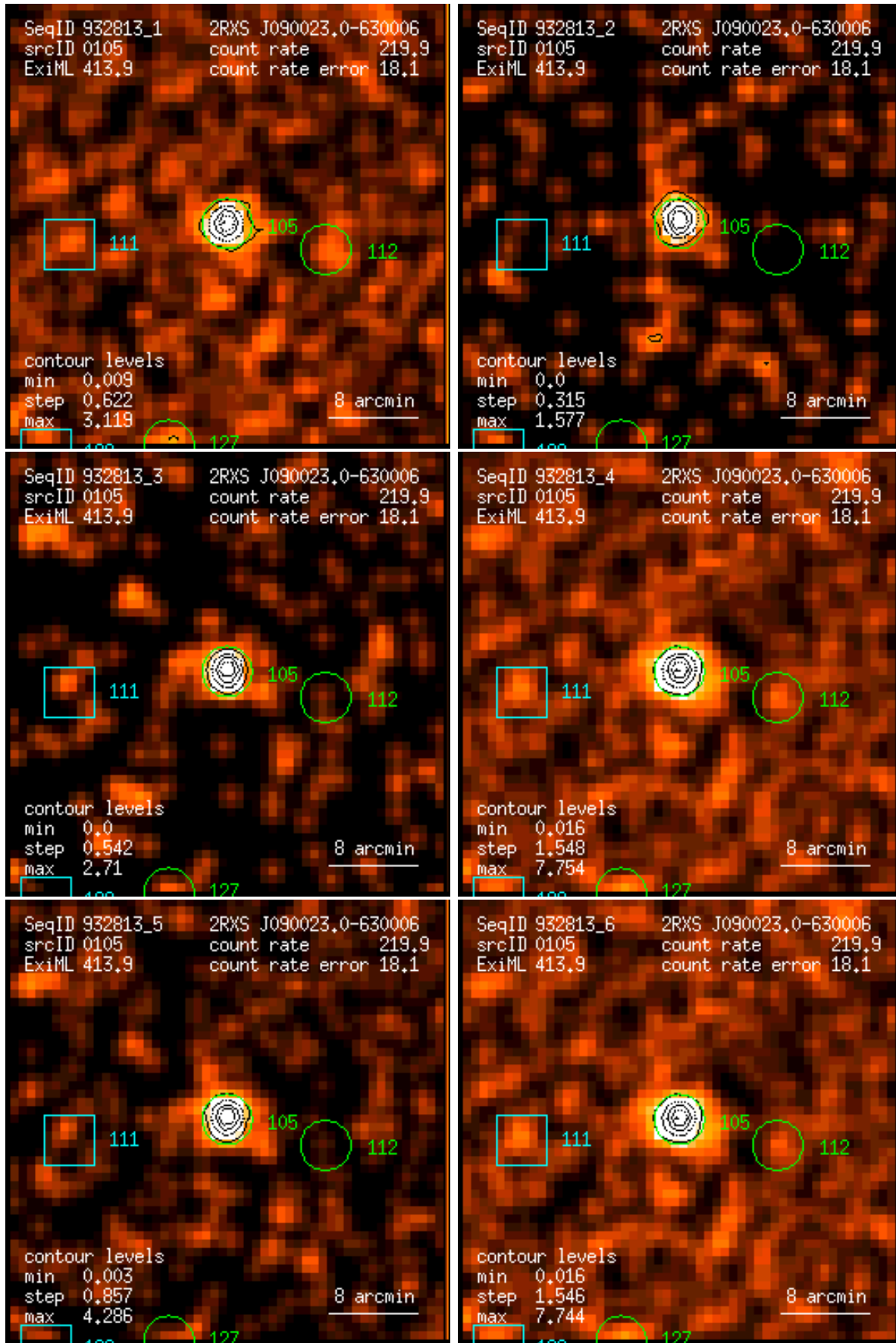
Figure 105: RASS 932813: detection 0105: band rate images, Gaussian filter: (1) PSPC channels 11 – 41, (2) 52 – 90, (3) 91 – 201, (4) 11 – 235, (5) 52 – 201, (6) 11 – 201. Broad band rates in counts/ks. Band rate contour levels in counts/ks/arcmin 2 .
