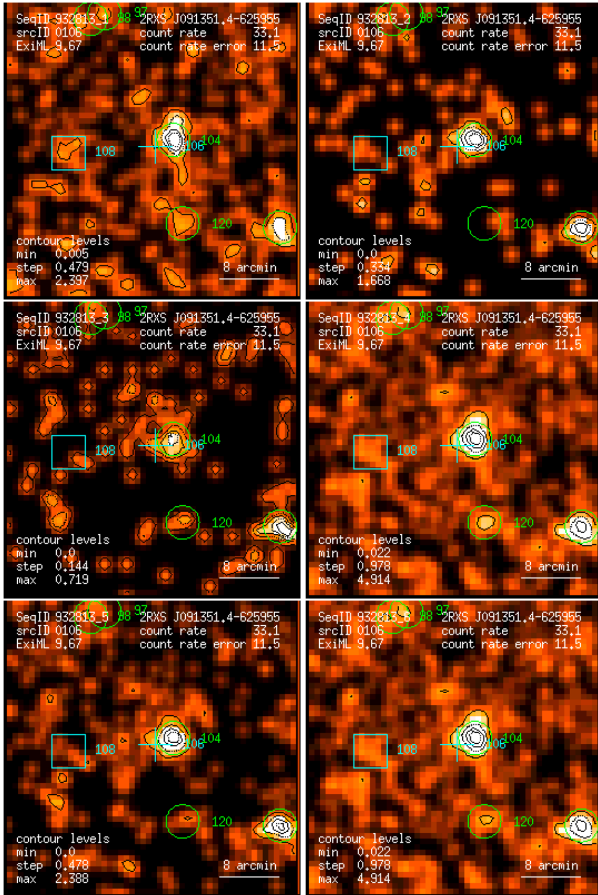
Figure 106: RASS 932813: detection 0106: band rate images, Gaussian filter: (1) PSPC channels 11 – 41, (2) 52 – 90, (3) 91 – 201, (4) 11 – 235, (5) 52 – 201, (6) 11 – 201. Broad band rates in counts/ks. Band rate contour levels in counts/ks/arcmin 2 .
