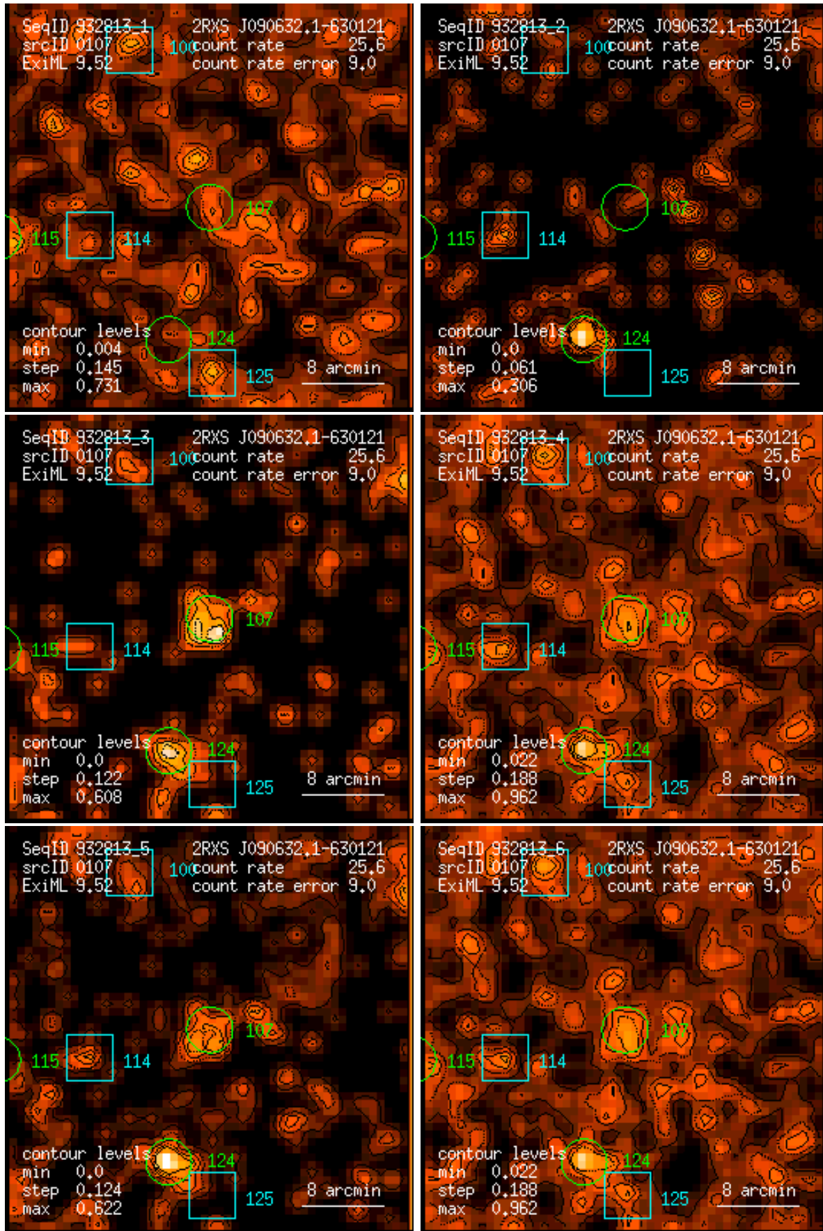
Figure 107: RASS 932813: detection 0107: band rate images, Gaussian filter: (1) PSPC channels 11 – 41, (2) 52 – 90, (3) 91 – 201, (4) 11 – 235, (5) 52 – 201, (6) 11 – 201. Broad band rates in counts/ks. Band rate contour levels in counts/ks/arcmin 2 .
