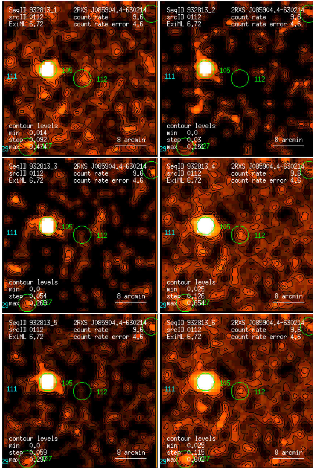
Figure 112: RASS 932813: detection 0112: band rate images, Gaussian filter: (1) PSPC channels 11 – 41, (2) 52 – 90, (3) 91 – 201, (4) 11 – 235, (5) 52 – 201, (6) 11 – 201. Broad band rates in counts/ks. Band rate contour levels in counts/ks/arcmin 2 .
