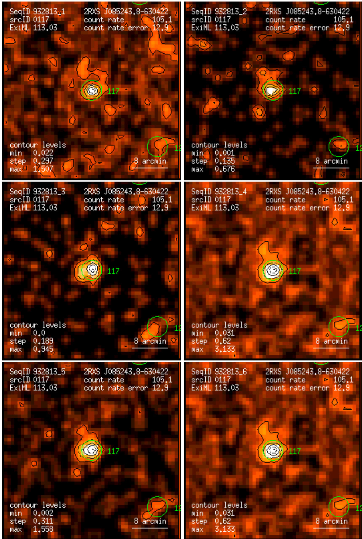
Figure 117: RASS 932813: detection 0117: band rate images, Gaussian filter: (1) PSPC channels 11 – 41, (2) 52 – 90, (3) 91 – 201, (4) 11 – 235, (5) 52 – 201, (6) 11 – 201. Broad band rates in counts/ks. Band rate contour levels in counts/ks/arcmin 2 .
