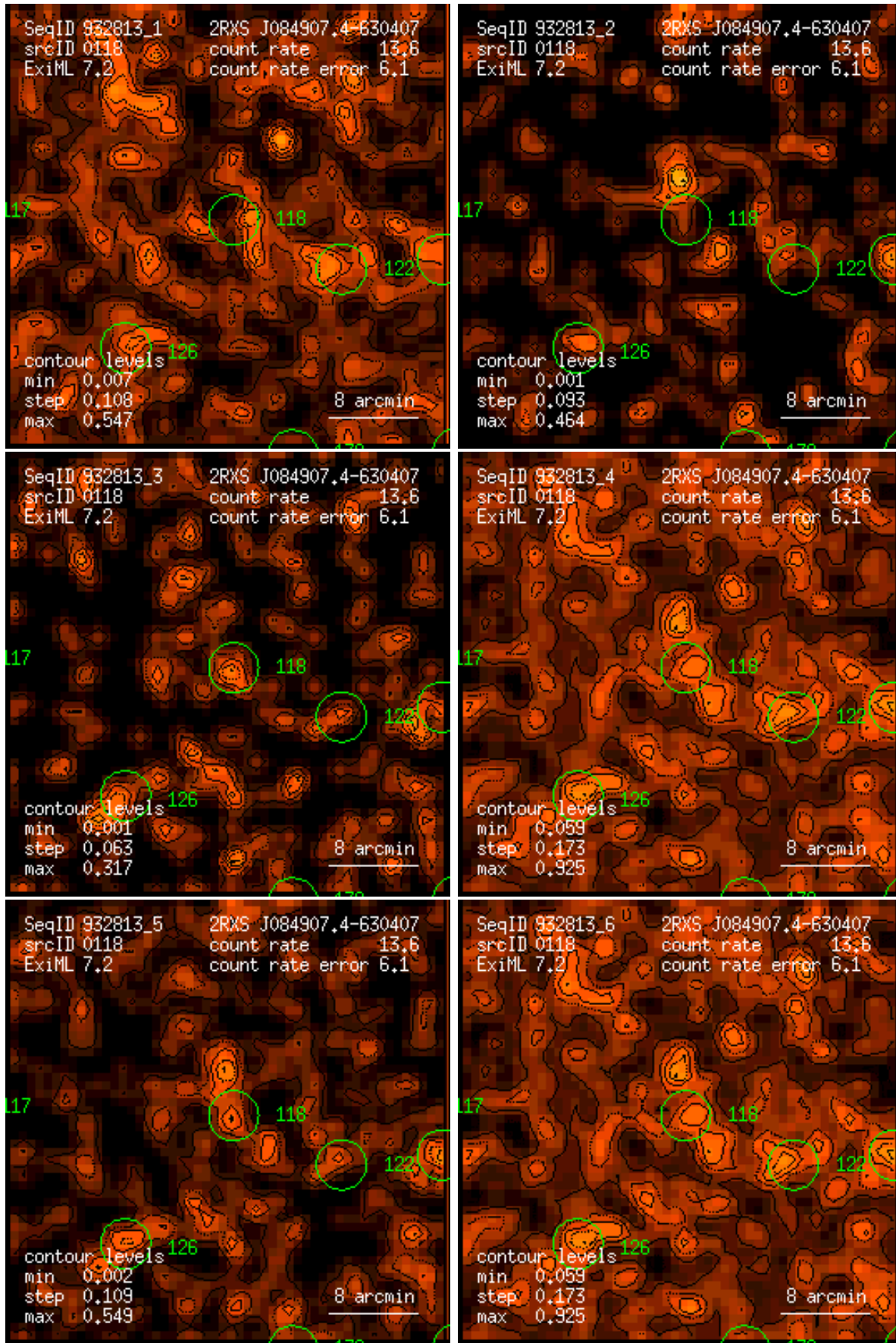
Figure 118: RASS 932813: detection 0118: band rate images, Gaussian filter: (1) PSPC channels 11 – 41, (2) 52 – 90, (3) 91 – 201, (4) 11 – 235, (5) 52 – 201, (6) 11 – 201. Broad band rates in counts/ks. Band rate contour levels in counts/ks/arcmin 2 .
