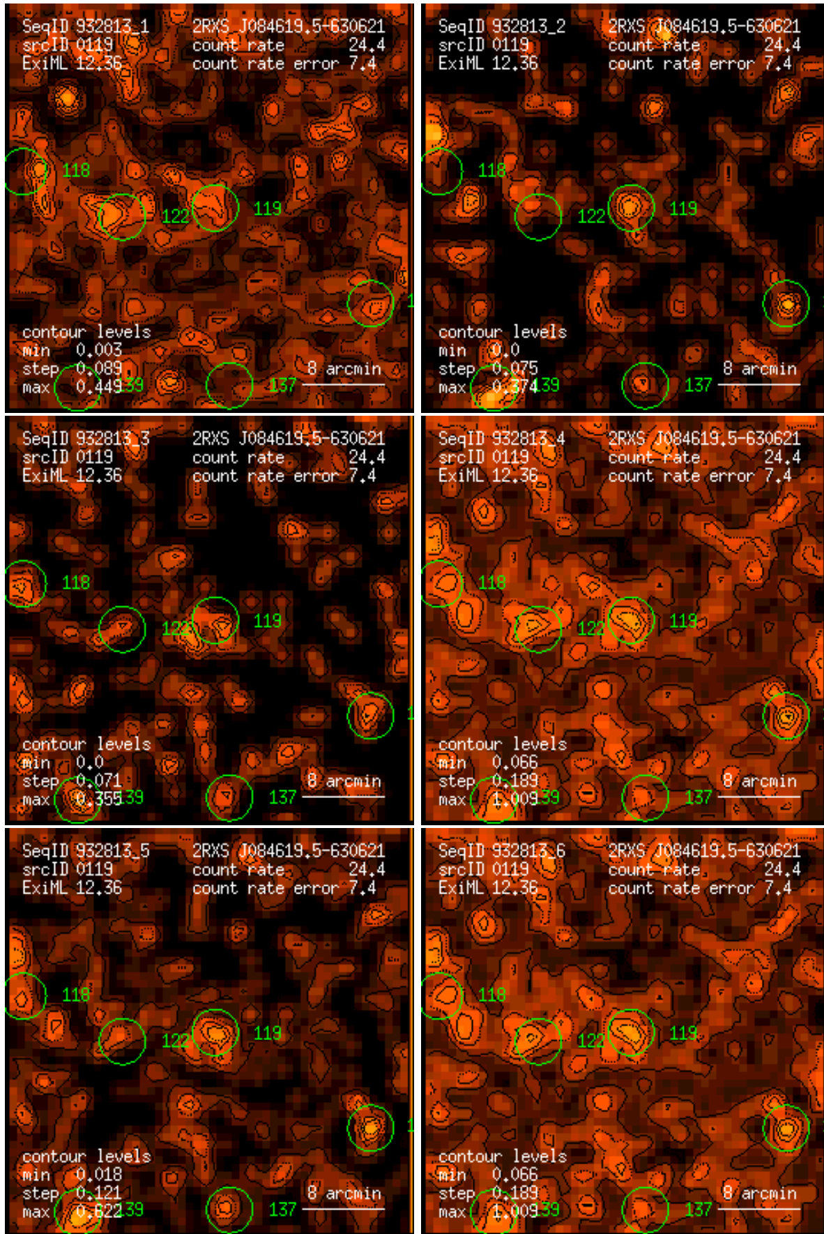
Figure 119: RASS 932813: detection 0119: band rate images, Gaussian filter: (1) PSPC channels 11 – 41, (2) 52 – 90, (3) 91 – 201, (4) 11 – 235, (5) 52 – 201, (6) 11 – 201. Broad band rates in counts/ks. Band rate contour levels in counts/ks/arcmin 2 .
