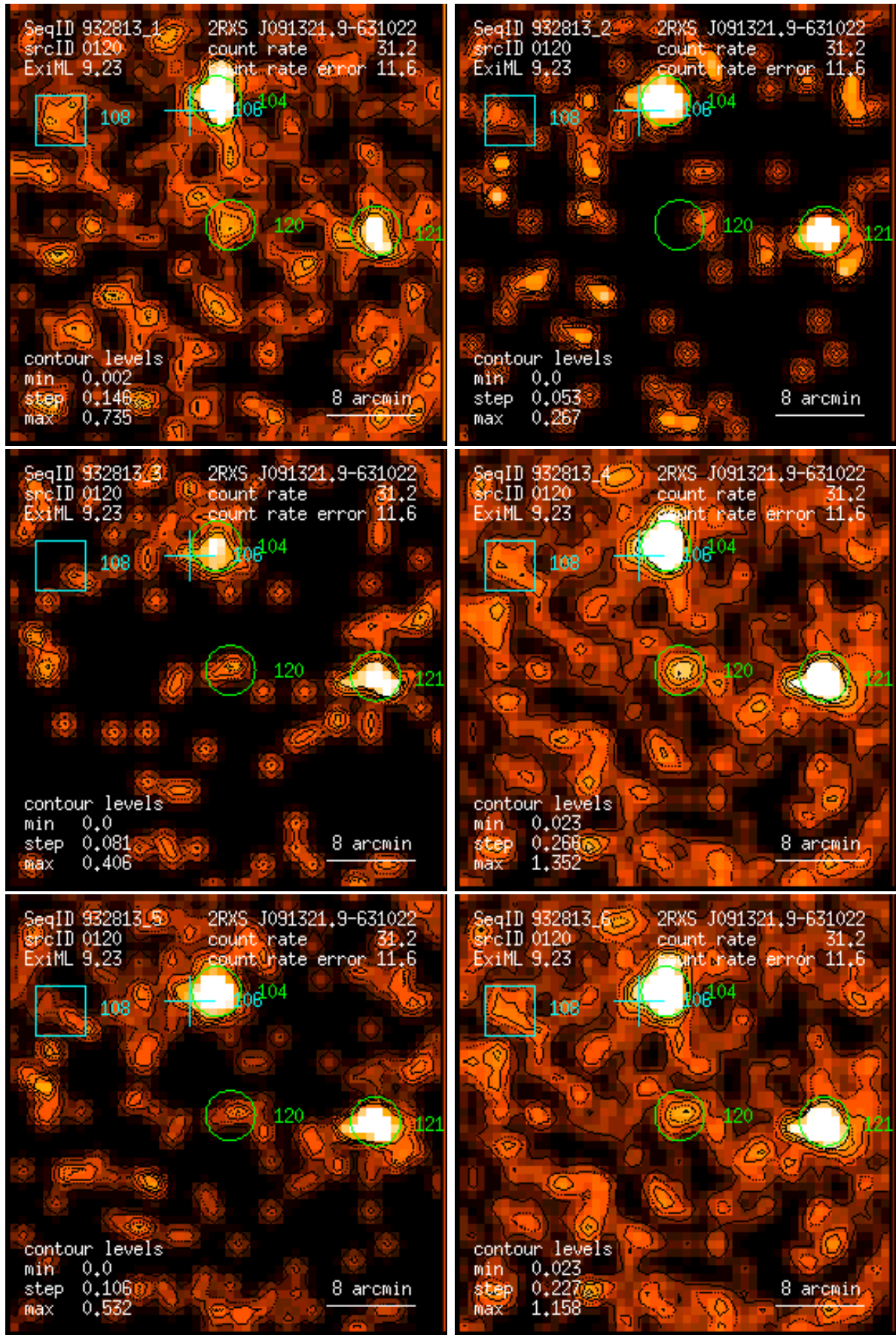
Figure 120: RASS 932813: detection 0120: band rate images, Gaussian filter: (1) PSPPC channels 11 – 41, (2) 52 – 90, (3) 91 – 201, (4) 11 – 235, (5) 52 – 201, (6) 11 – 201. Broad band rates in counts/ks. Band rate contour levels in counts/ks/arcmin 2 .
