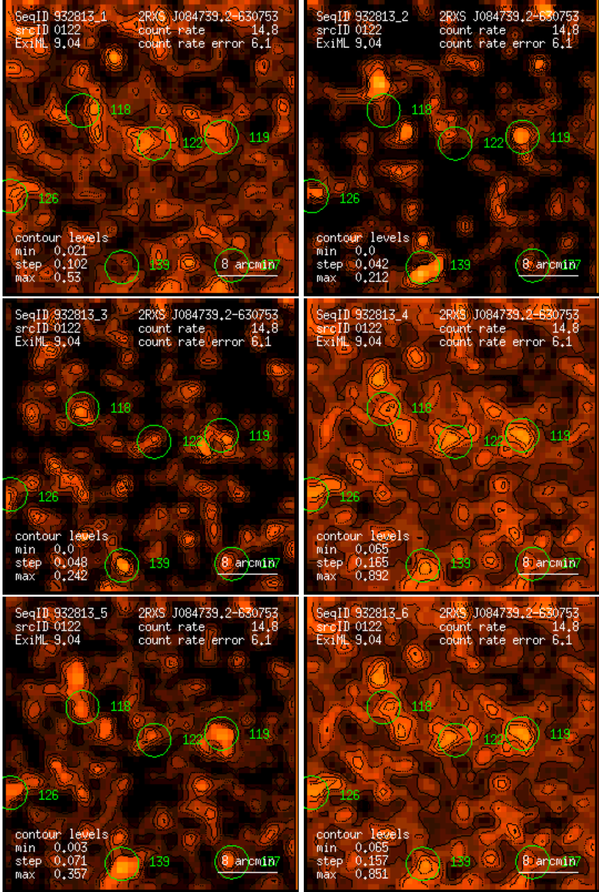
Figure 122: RASS 932813: detection 0122: band rate images, Gaussian filter: (1) PSPC channels 11 – 41, (2) 52 – 90, (3) 91 – 201, (4) 11 – 235, (5) 52 – 201, (6) 11 – 201. Broad band rates in counts/ks. Band rate contour levels in counts/ks/arcmin 2 .
