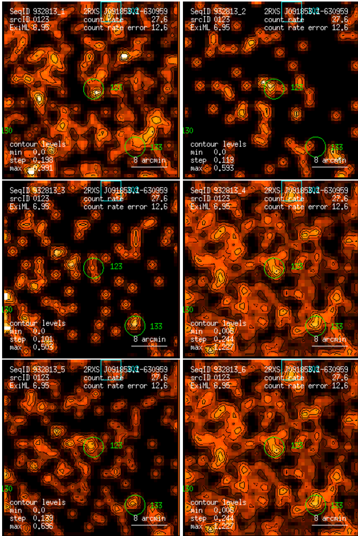
Figure 123: RASS 932813: detection 0123: band rate images, Gaussian filter: (1) PSPC channels 11 – 41, (2) 52 – 90, (3) 91 – 201, (4) 11 – 235, (5) 52 – 201, (6) 11 – 201. Broad band rates in counts/ks. Band rate contour levels in counts/ks/arcmin 2 .
