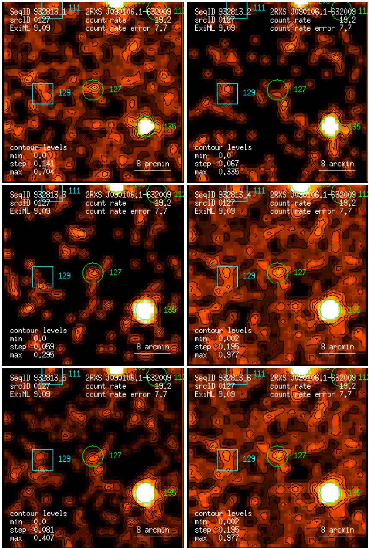
Figure 127: RASS 932813: detection 0127: band rate images, Gaussian filter: (1) PSPC channels 11 – 41, (2) 52 – 90, (3) 91 – 201, (4) 11 – 235, (5) 52 – 201, (6) 11 – 201. Broad band rates in counts/ks. Band rate contour levels in counts/ks/arcmin 2 .
