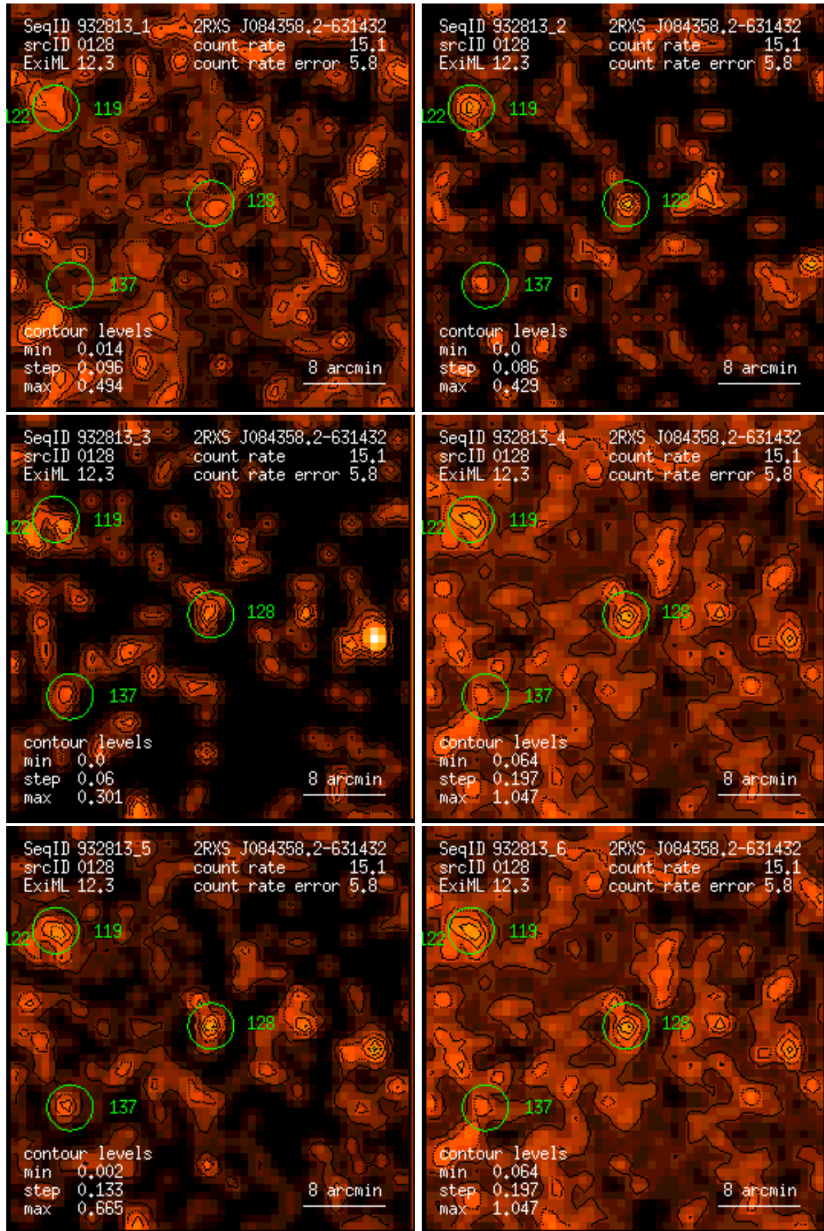
Figure 128: RASS 932813: detection 0128: band rate images, Gaussian filter: (1) PSPC channels 11 – 41, (2) 52 – 90, (3) 91 – 201, (4) 11 – 235, (5) 52 – 201, (6) 11 – 201. Broad band rates in counts/ks. Band rate contour levels in counts/ks/arcmin 2 .
