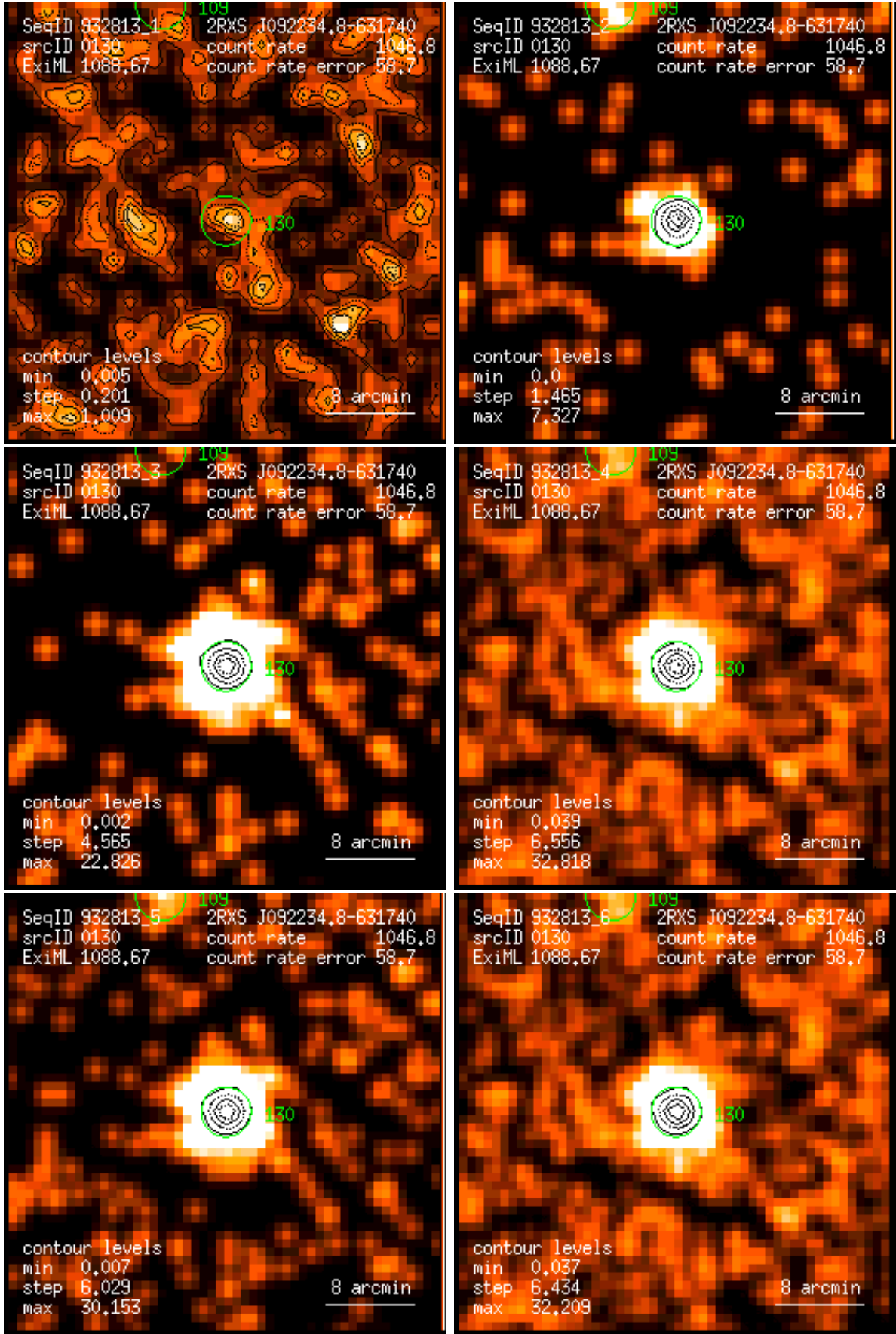
Figure 130: RASS 932813: detection 0130: band rate images, Gaussian filter: (1) PSPC channels 11 – 41, (2) 52 – 90, (3) 91 – 201, (4) 11 – 235, (5) 52 – 201, (6) 11 – 201. Broad band rates in counts/ks. Band rate contour levels in counts/ks/arcmin 2 .
