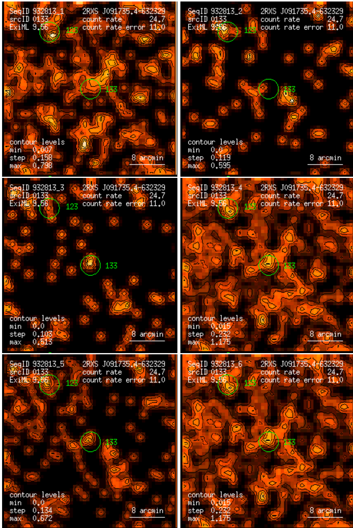
Figure 133: RASS 932813: detection 0133: band rate images, Gaussian filter: (1) PSPC channels 11 – 41, (2) 52 – 90, (3) 91 – 201, (4) 11 – 235, (5) 52 – 201, (6) 11 – 201. Broad band rates in counts/ks. Band rate contour levels in counts/ks/arcmin 2 .
