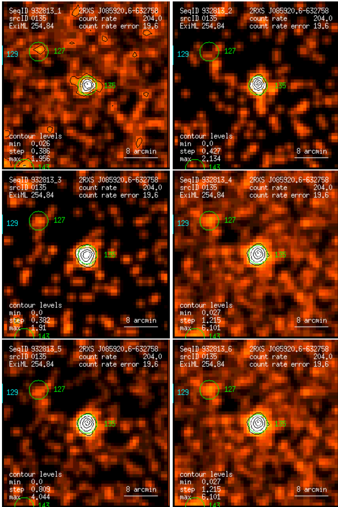
Figure 135: RASS 932813: detection 0135: band rate images, Gaussian filter: (1) PSPC channels 11 – 41, (2) 52 – 90, (3) 91 – 201, (4) 11 – 235, (5) 52 – 201, (6) 11 – 201. Broad band rates in counts/ks. Band rate contour levels in counts/ks/arcmin 2 .
