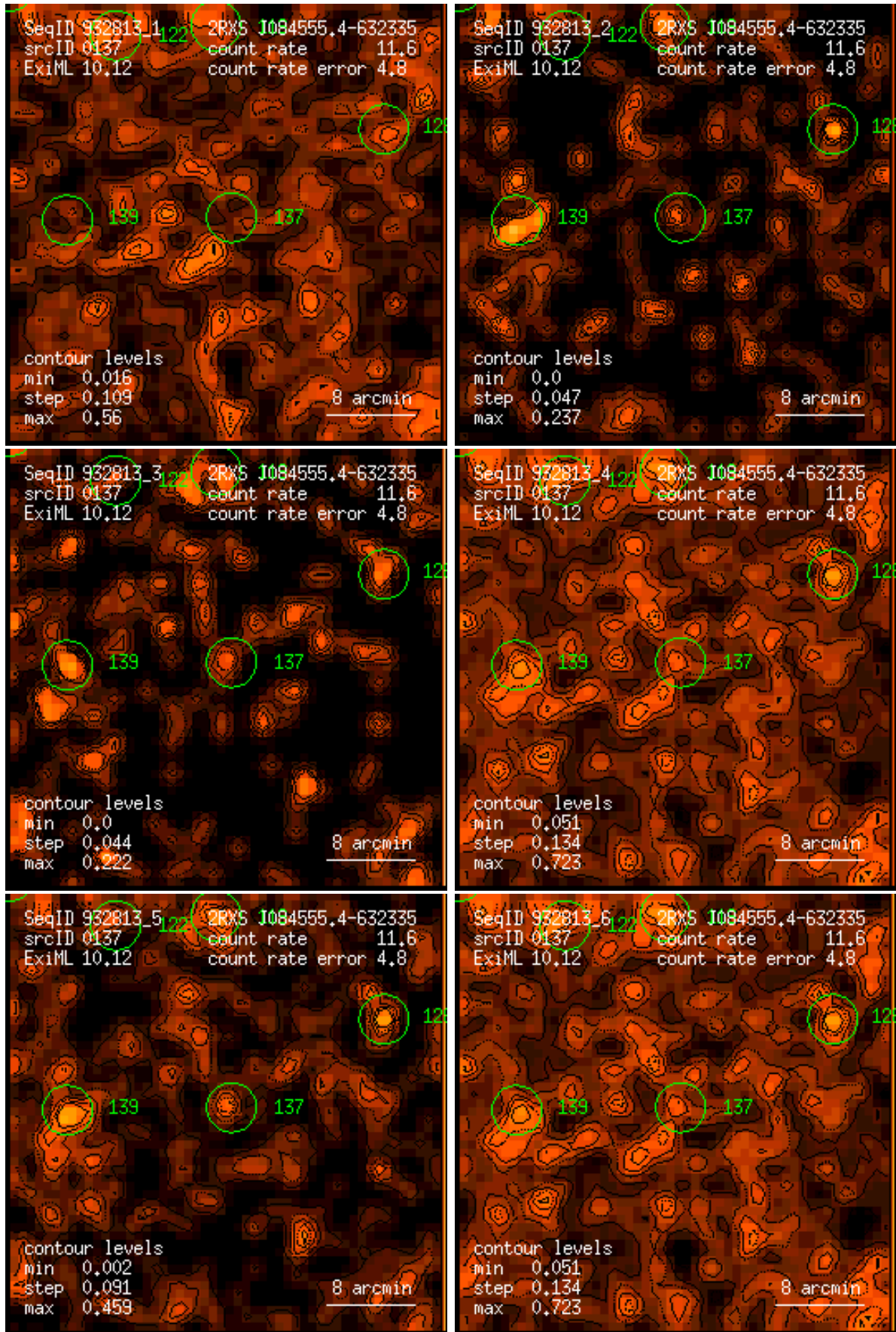
Figure 137: RASS 932813: detection 0137: band rate images, Gaussian filter: (1) PSPC channels 11 – 41, (2) 52 – 90, (3) 91 – 201, (4) 11 – 235, (5) 52 – 201, (6) 11 – 201. Broad band rates in counts/ks. Band rate contour levels in counts/ks/arcmin 2 .
