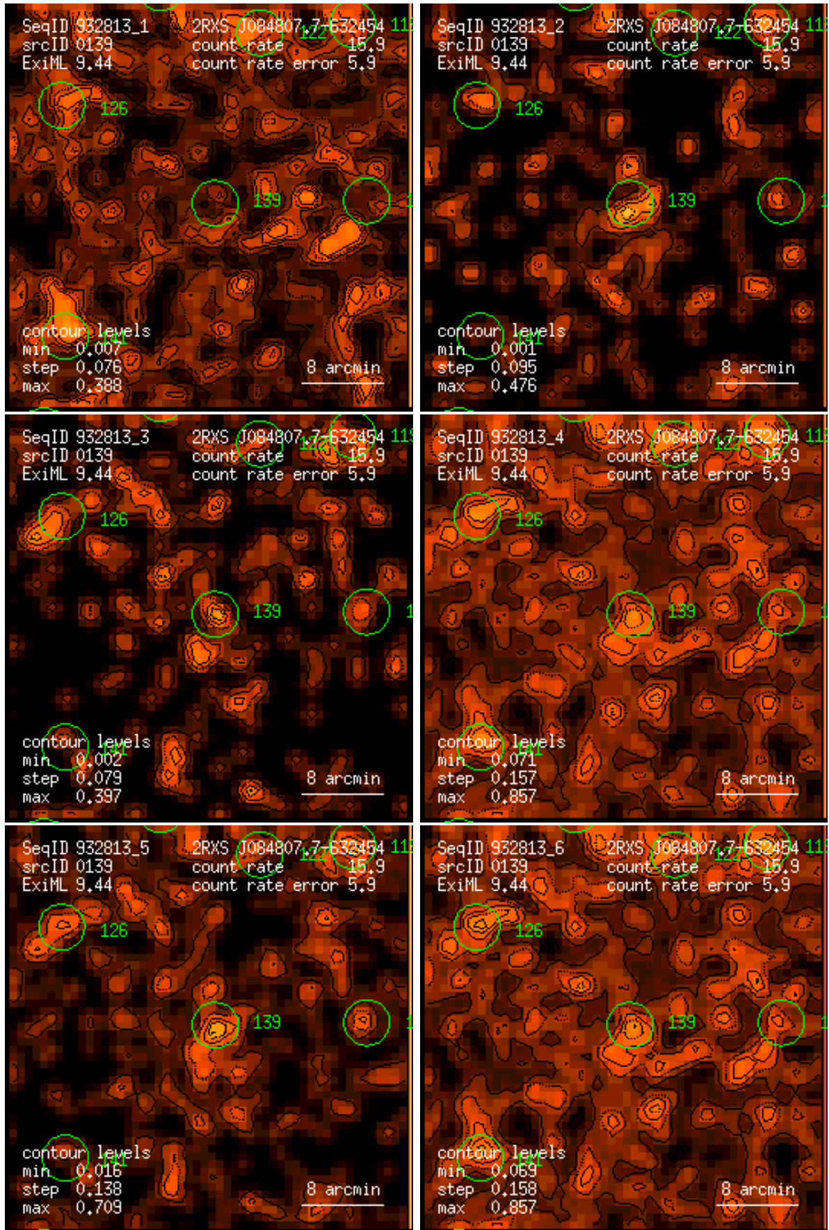
Figure 139: RASS 932813: detection 0139: band rate images, Gaussian filter: (1) PSPC channels 11 – 41, (2) 52 – 90, (3) 91 – 201, (4) 11 – 235, (5) 52 – 201, (6) 11 – 201. Broad band rates in counts/ks. Band rate contour levels in counts/ks/arcmin 2 .
