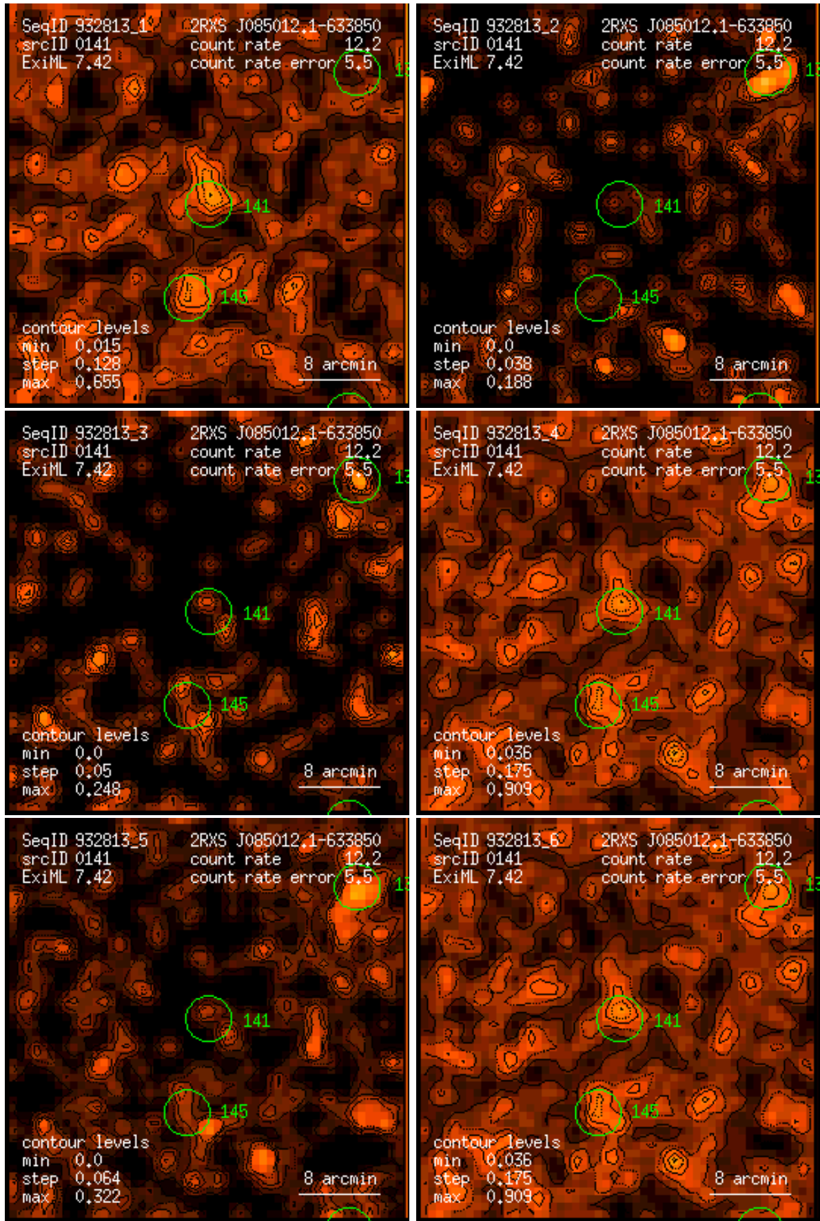
Figure 141: RASS 932813: detection 0141: band rate images, Gaussian filter: (1) PSPC channels 11 – 41, (2) 52 – 90, (3) 91 – 201, (4) 11 – 235, (5) 52 – 201, (6) 11 – 201. Broad band rates in counts/ks. Band rate contour levels in counts/ks/arcmin 2 .
