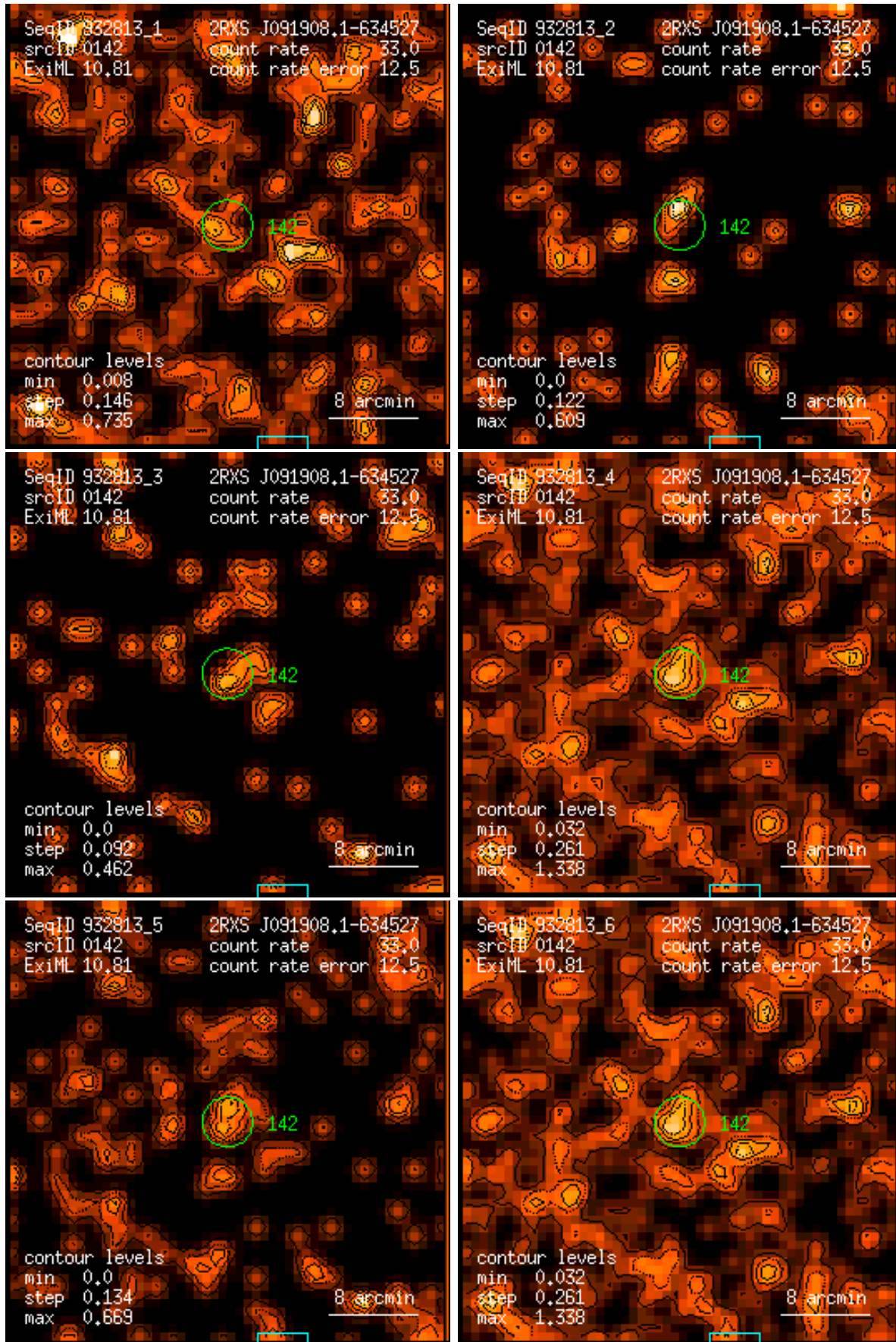
Figure 142: RASS 932813: detection 0142: band rate images, Gaussian filter: (1) PSPC channels 11 – 41, (2) 52 – 90, (3) 91 – 201, (4) 11 – 235, (5) 52 – 201, (6) 11 – 201. Broad band rates in counts/ks. Band rate contour levels in counts/ks/arcmin 2 .
