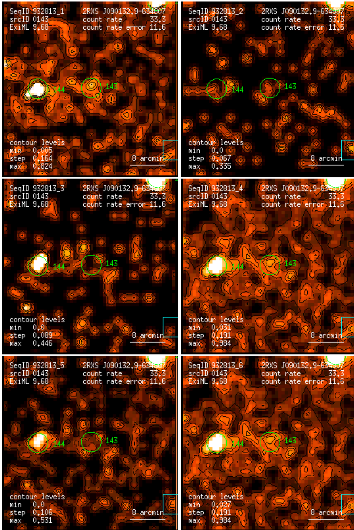
Figure 143: RASS 932813: detection 0143: band rate images, Gaussian filter: (1) PSPC channels 11 – 41, (2) 52 – 90, (3) 91 – 201, (4) 11 – 235, (5) 52 – 201, (6) 11 – 201. Broad band rates in counts/ks. Band rate contour levels in counts/ks/arcmin 2 .
