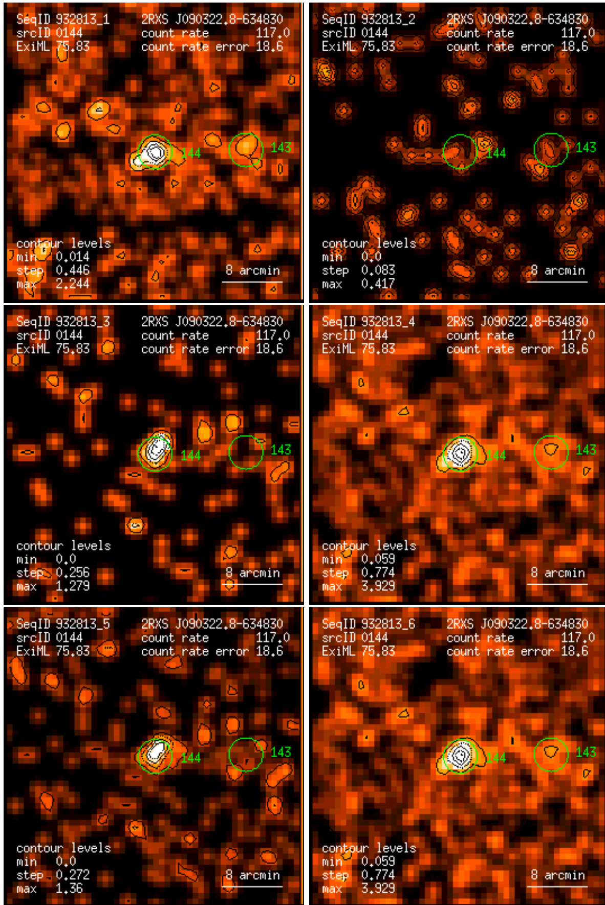
Figure 144: RASS 932813: detection 0144: band rate images, Gaussian filter: (1) PSPC channels 11 – 41, (2) 52 – 90, (3) 91 – 201, (4) 11 – 235, (5) 52 – 201, (6) 11 – 201. Broad band rates in counts/ks. Band rate contour levels in counts/ks/arcmin 2 .
