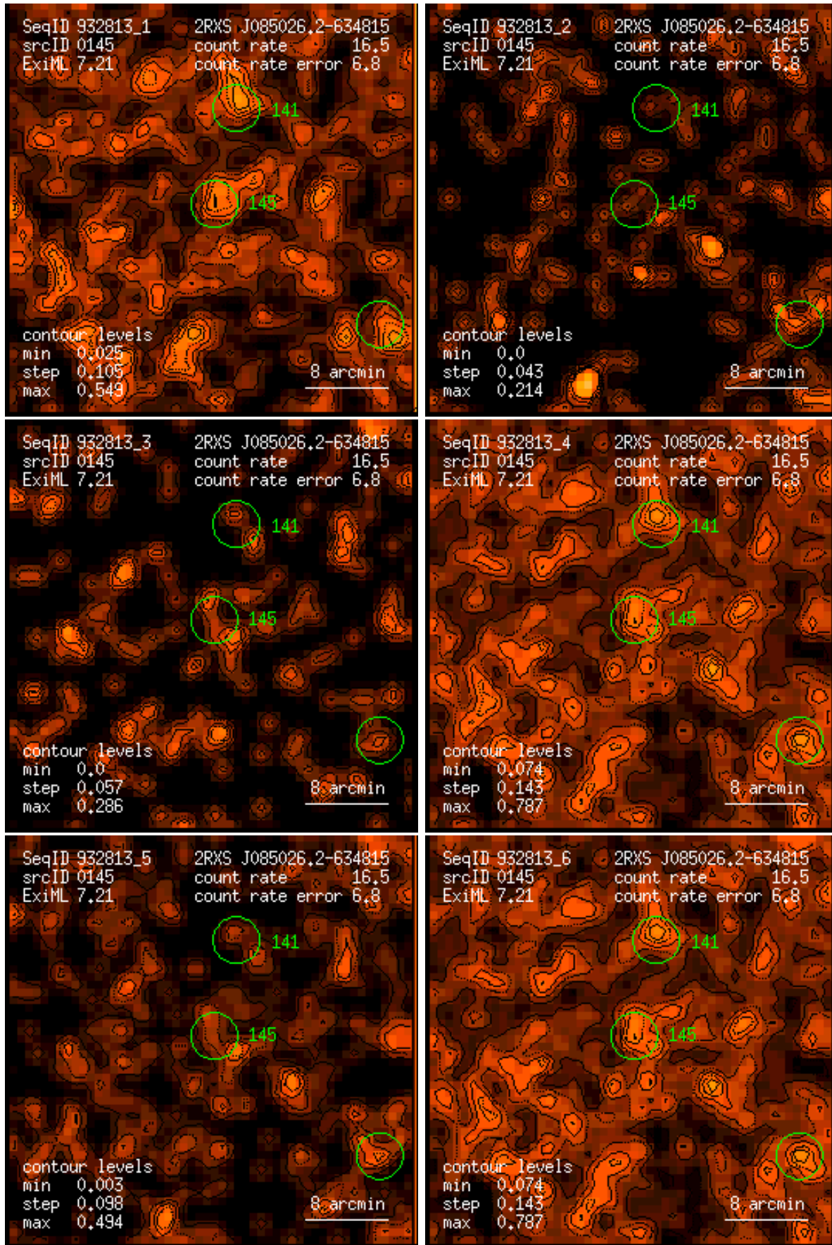
Figure 145: RASS 932813: detection 0145: band rate images, Gaussian filter: (1) PSPC channels 11 – 41, (2) 52 – 90, (3) 91 – 201, (4) 11 – 235, (5) 52 – 201, (6) 11 – 201. Broad band rates in counts/ks. Band rate contour levels in counts/ks/arcmin 2 .
