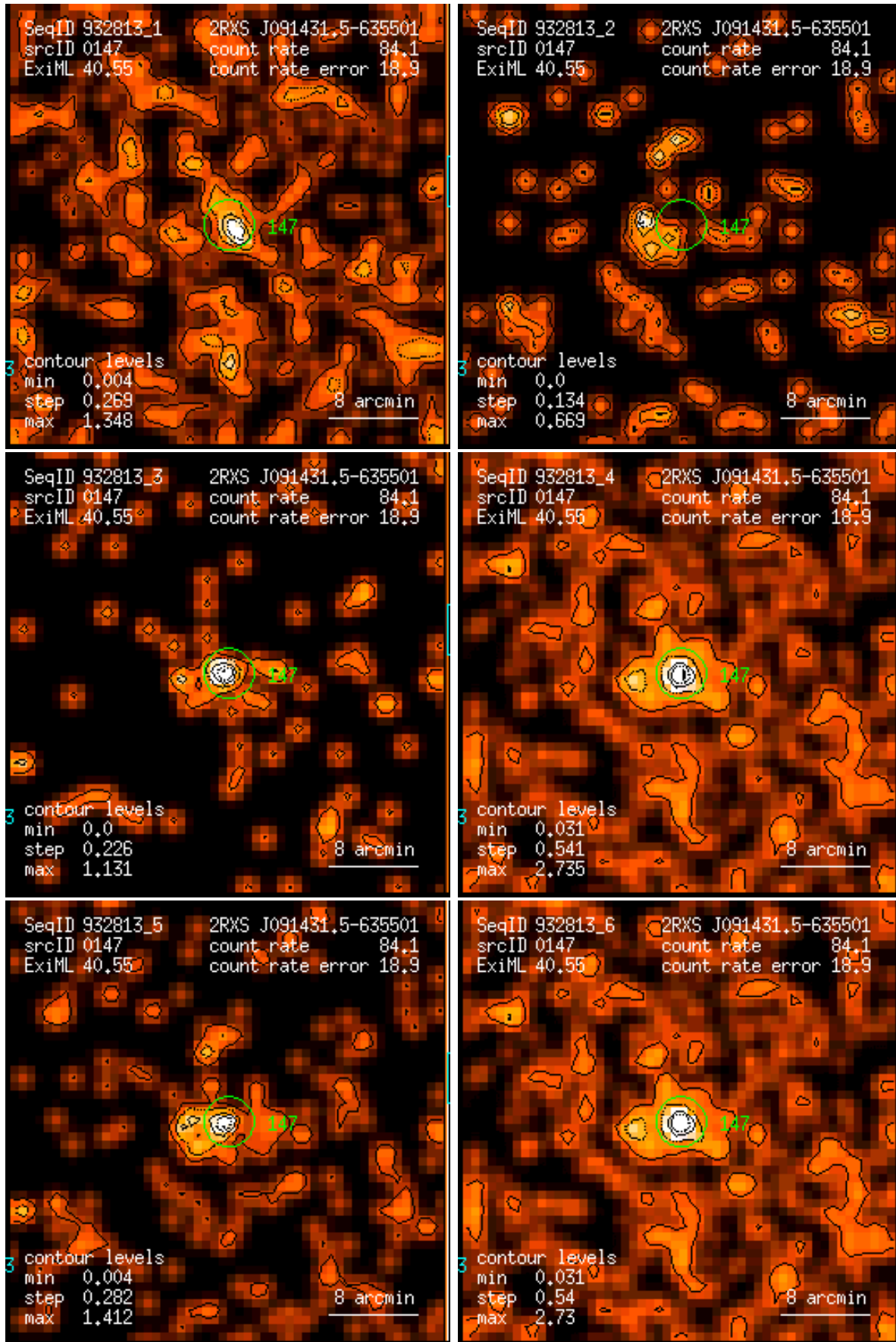
Figure 147: RASS 932813: detection 0147: band rate images, Gaussian filter: (1) PSPC channels 11 – 41, (2) 52 – 90, (3) 91 – 201, (4) 11 – 235, (5) 52 – 201, (6) 11 – 201. Broad band rates in counts/ks. Band rate contour levels in counts/ks/arcmin 2 .
