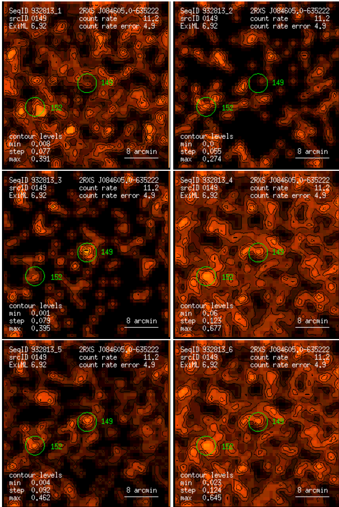
Figure 149: RASS 932813: detection 0149: band rate images, Gaussian filter: (1) PSPC channels 11 – 41, (2) 52 – 90, (3) 91 – 201, (4) 11 – 235, (5) 52 – 201, (6) 11 – 201. Broad band rates in counts/ks. Band rate contour levels in counts/ks/arcmin 2 .
