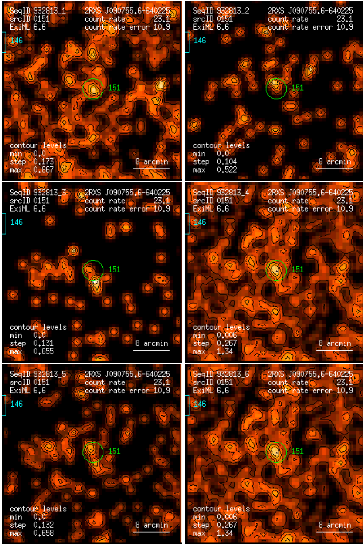
Figure 151: RASS 932813: detection 0151: band rate images, Gaussian filter: (1) PSPC channels 11 – 41, (2) 52 – 90, (3) 91 – 201, (4) 11 – 235, (5) 52 – 201, (6) 11 – 201. Broad band rates in counts/ks. Band rate contour levels in counts/ks/arcmin 2 .
