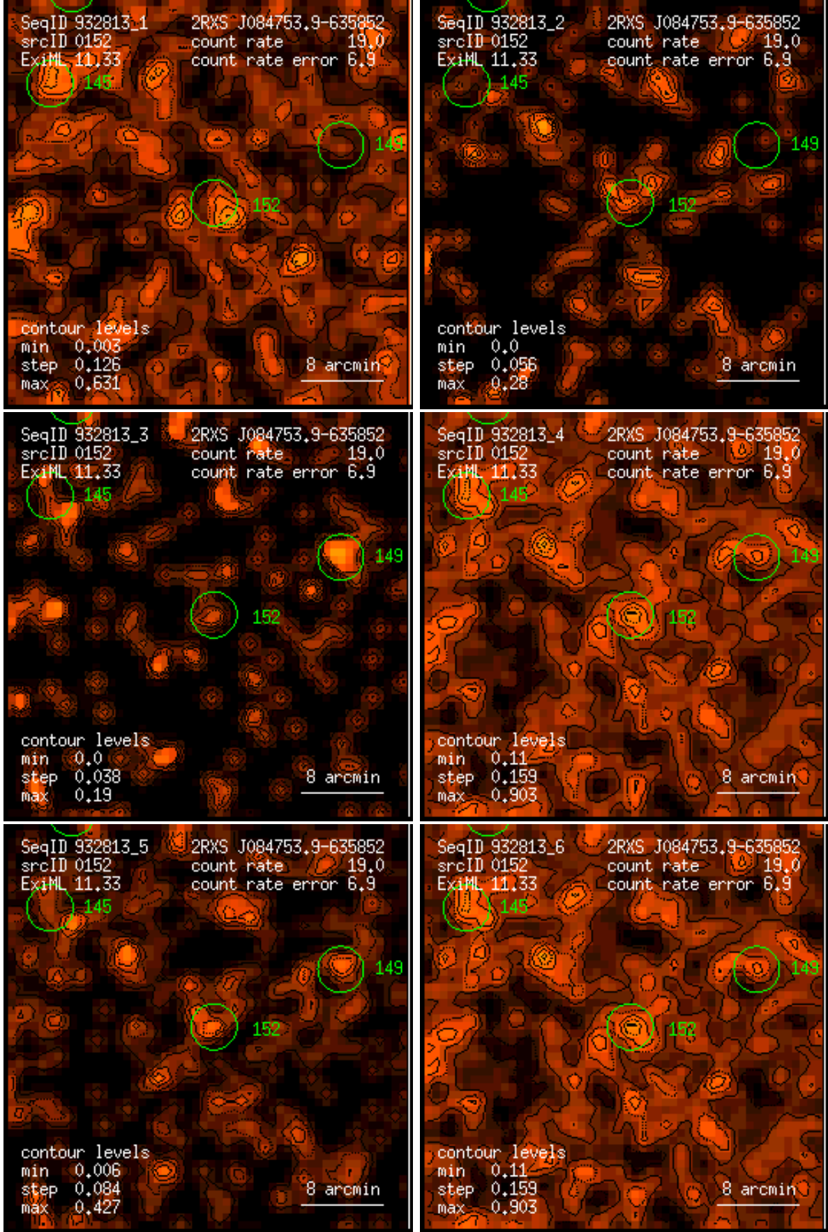
Figure 152: RASS 932813: detection 0152: band rate images, Gaussian filter: (1) PSPC channels 11 – 41, (2) 52 – 90, (3) 91 – 201, (4) 11 – 235, (5) 52 – 201, (6) 11 – 201. Broad band rates in counts/ks. Band rate contour levels in counts/ks/arcmin 2 .
