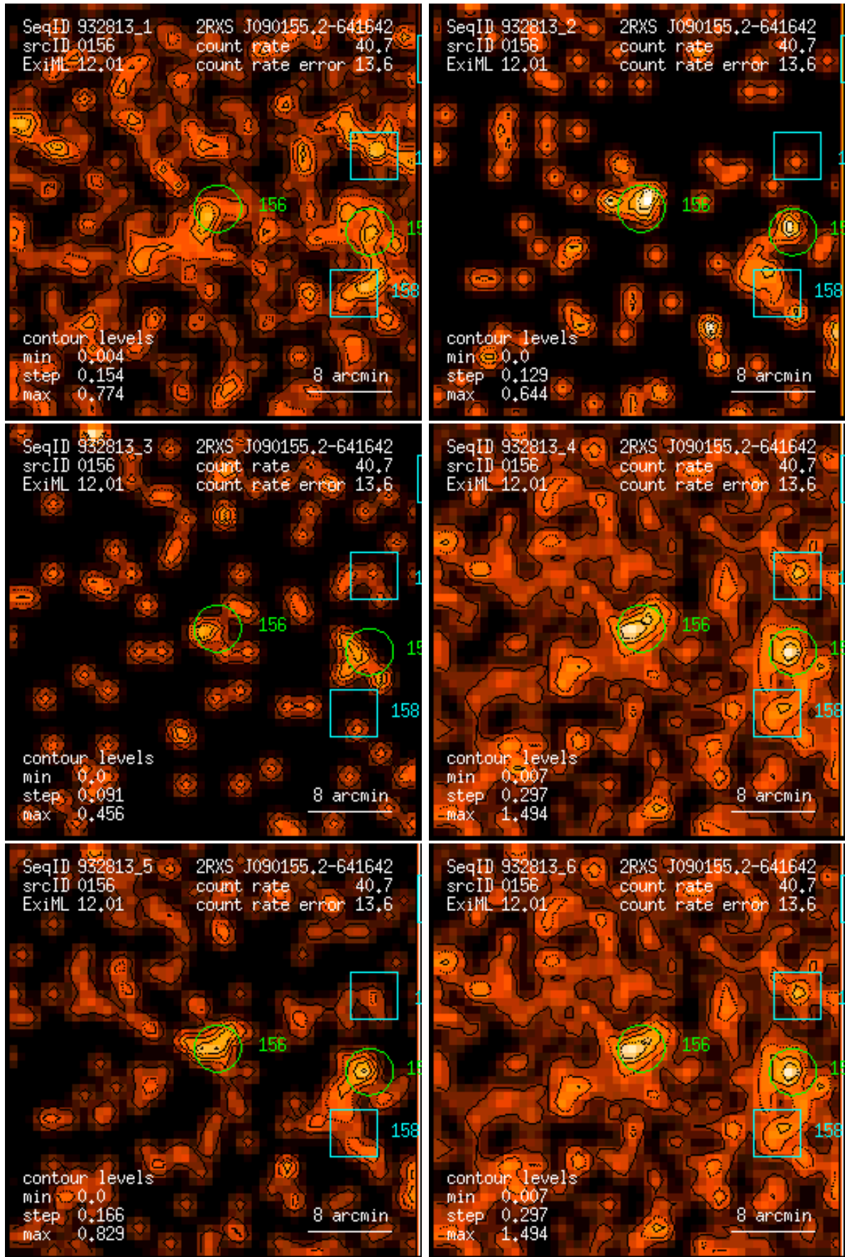
Figure 156: RASS 932813: detection 0156: band rate images, Gaussian filter: (1) PSPC channels 11 – 41, (2) 52 – 90, (3) 91 – 201, (4) 11 – 235, (5) 52 – 201, (6) 11 – 201. Broad band rates in counts/ks. Band rate contour levels in counts/ks/arcmin 2 .
