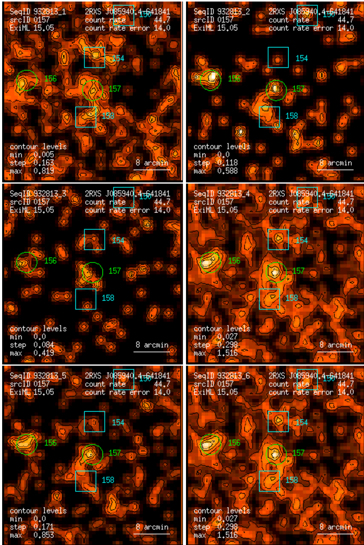
Figure 157: RASS 932813: detection 0157: band rate images, Gaussian filter: (1) PSPC channels 11 – 41, (2) 52 – 90, (3) 91 – 201, (4) 11 – 235, (5) 52 – 201, (6) 11 – 201. Broad band rates in counts/ks. Band rate contour levels in counts/ks/arcmin 2 .
