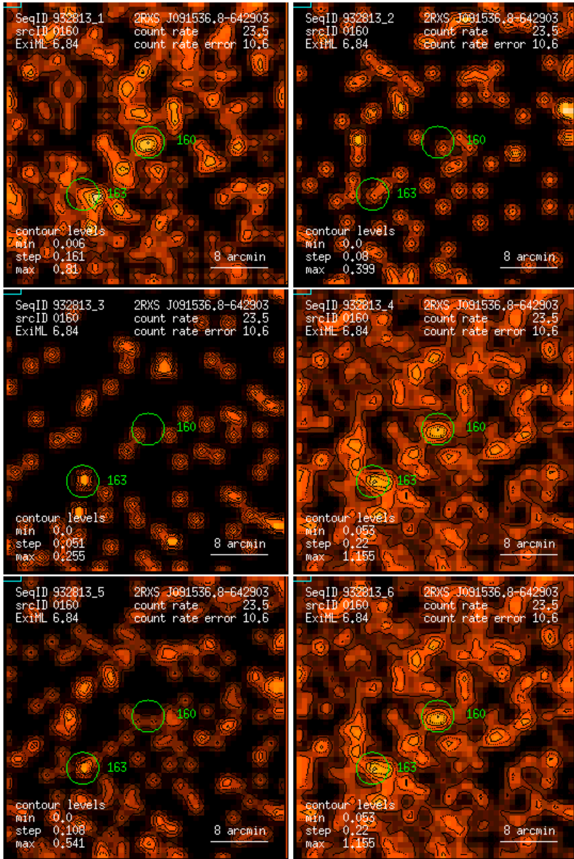
Figure 160: RASS 932813: detection 0160: band rate images, Gaussian filter: (1) PSPC channels 11 – 41, (2) 52 – 90, (3) 91 – 201, (4) 11 – 235, (5) 52 – 201, (6) 11 – 201. Broad band rates in counts/ks. Band rate contour levels in counts/ks/arcmin 2 .
