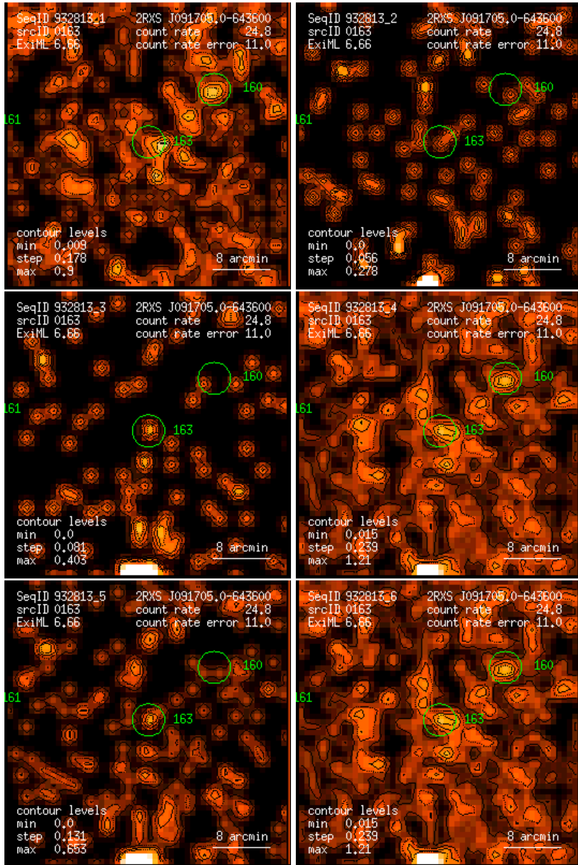
Figure 163: RASS 932813: detection 0163: band rate images, Gaussian filter: (1) PSPC channels 11 – 41, (2) 52 – 90, (3) 91 – 201, (4) 11 – 235, (5) 52 – 201, (6) 11 – 201. Broad band rates in counts/ks. Band rate contour levels in counts/ks/arcmin 2 .
