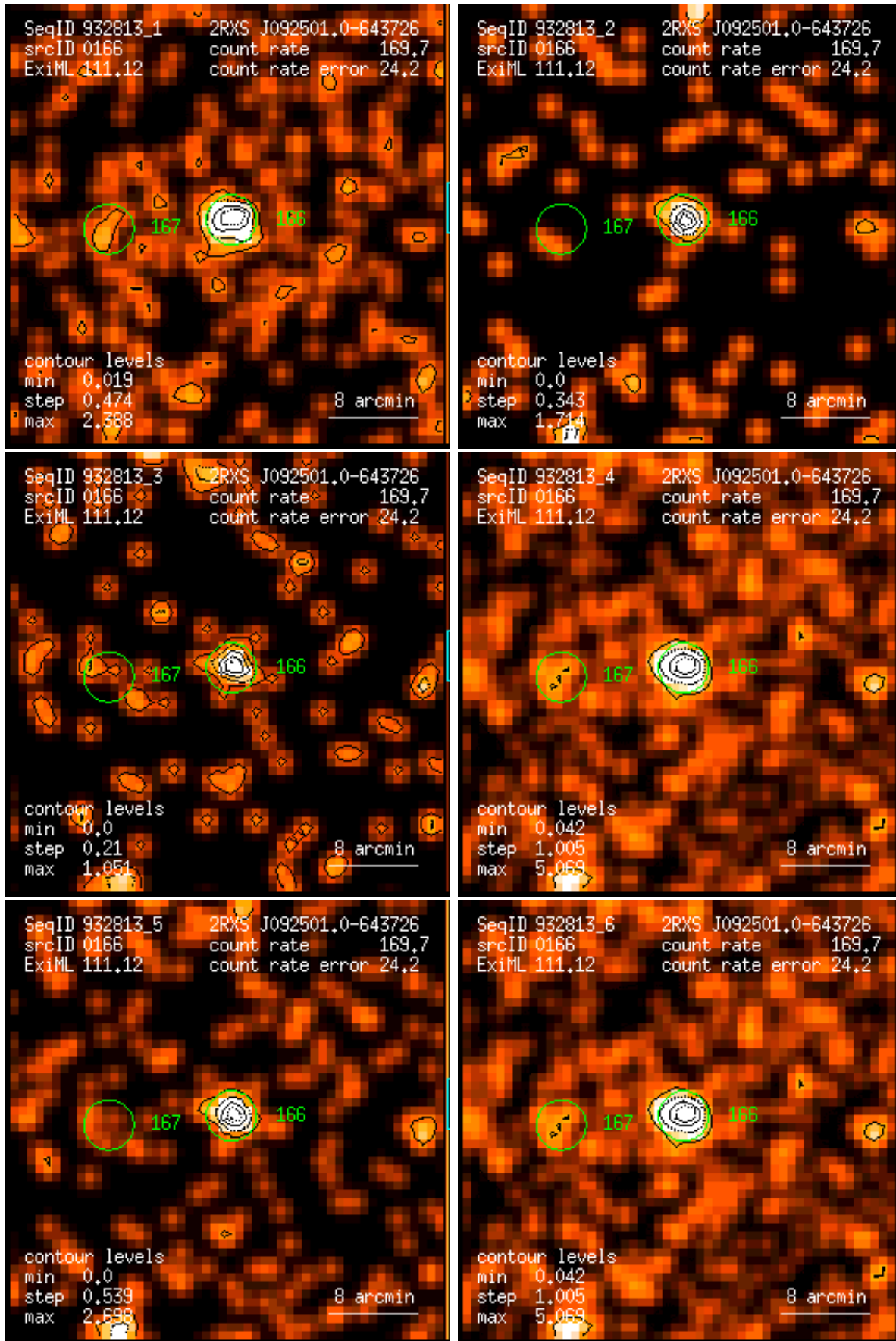
Figure 166: RASS 932813: detection 0166: band rate images, Gaussian filter: (1) PSPC channels 11 – 41, (2) 52 – 90, (3) 91 – 201, (4) 11 – 235, (5) 52 – 201, (6) 11 – 201. Broad band rates in counts/ks. Band rate contour levels in counts/ks/arcmin 2 .
