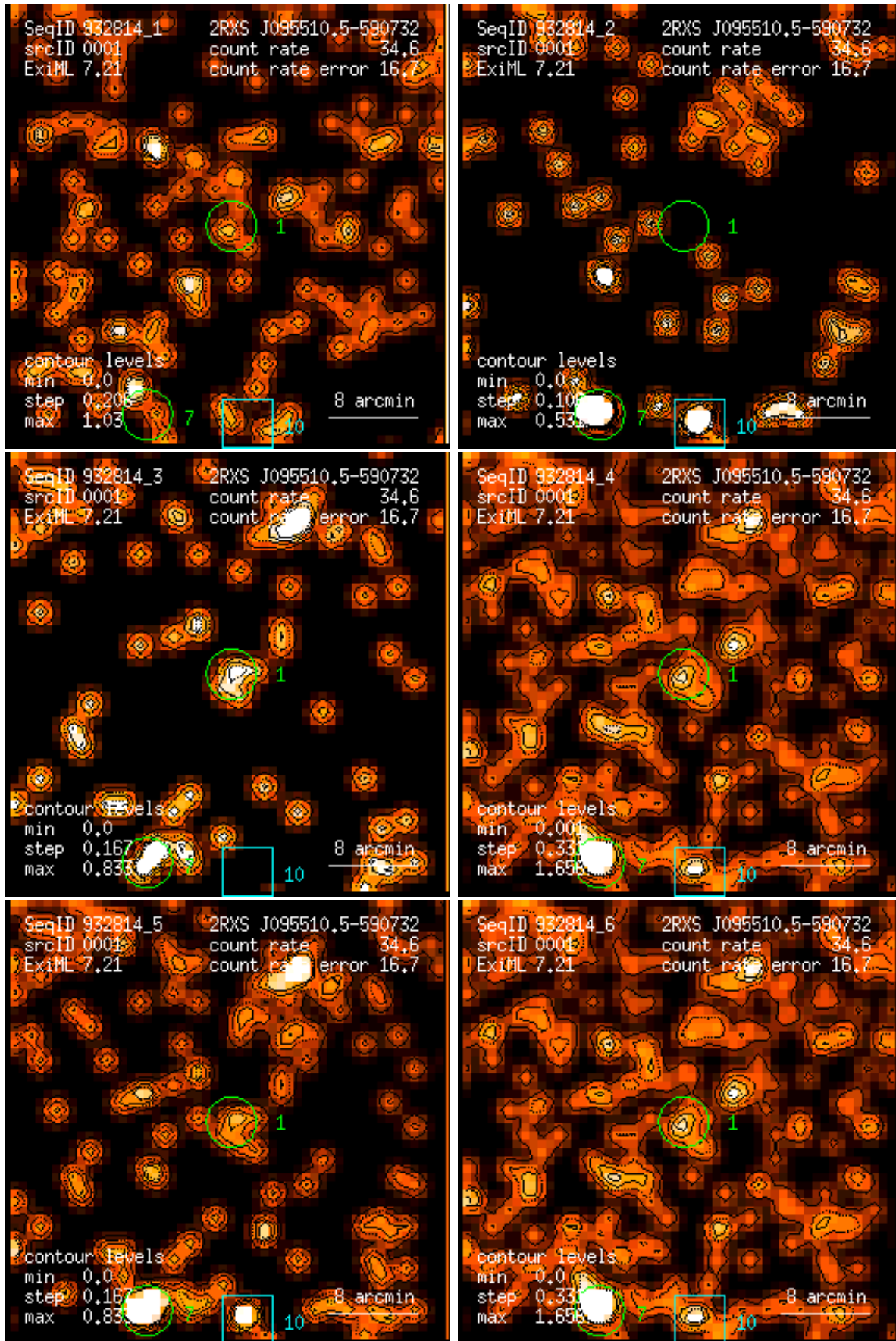
Figure 1: RASS 932814: detection 0001: band rate images, Gaussian filter: (1) PSPC channels 11 – 41, (2) 52 – 90, (3) 91 – 201, (4) 11 – 235, (5) 52 – 201, (6) 11 – 201. Broad band rates in counts/ks. Band rate contour levels in counts/ks/arcmin 2 .
