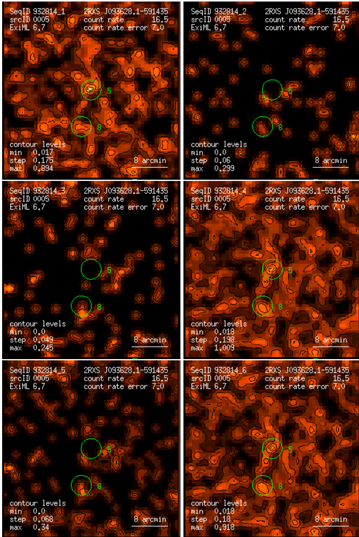
Figure 5: RASS 932814: detection 0005: band rate images, Gaussian filter: (1) PSPC channels 11 – 41, (2) 52 – 90, (3) 91 – 201, (4) 11 – 235, (5) 52 – 201, (6) 11 – 201. Broad band rates in counts/ks. Band rate contour levels in counts/ks/arcmin 2 .
