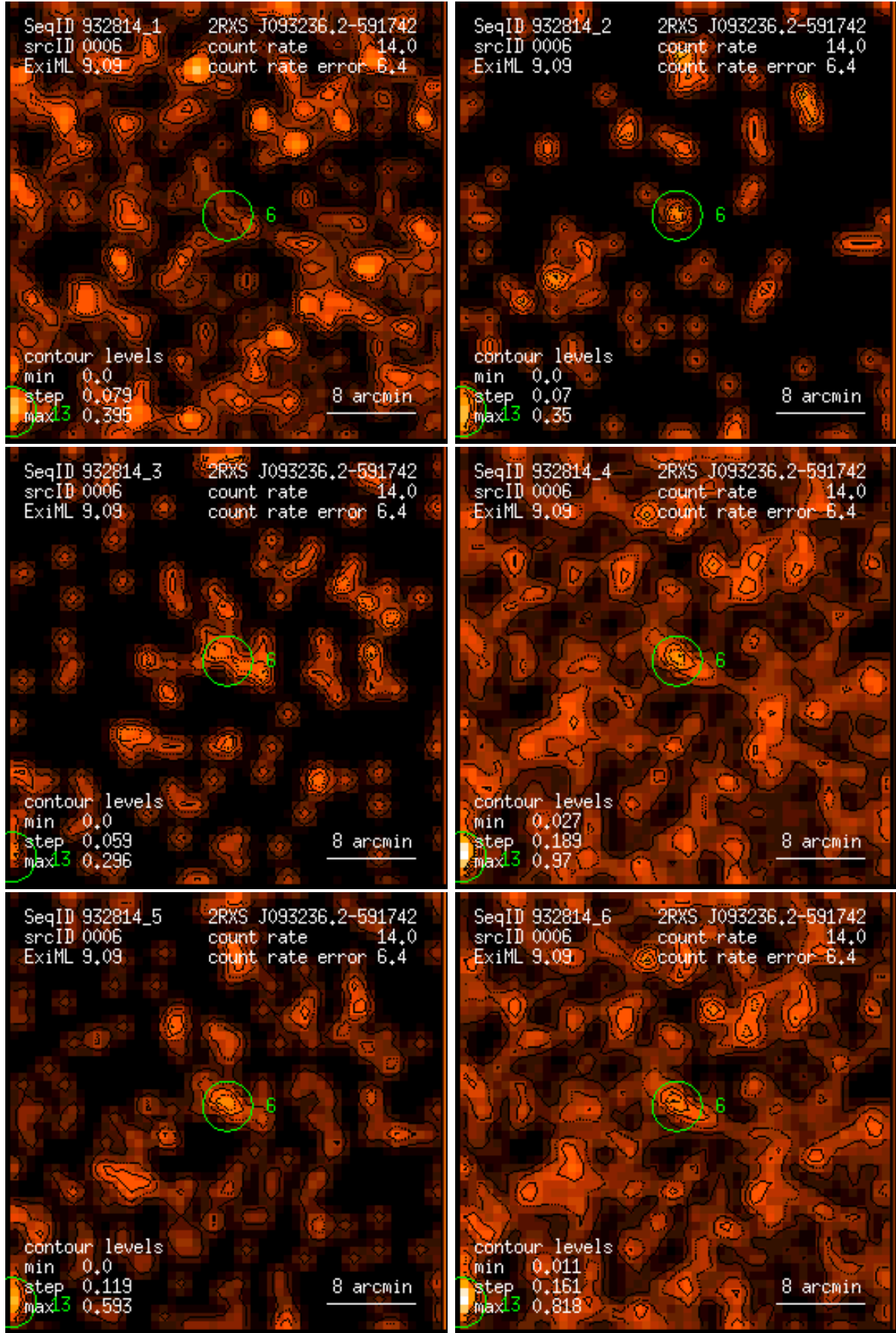
Figure 6: RASS 932814: detection 0006: band rate images, Gaussian filter: (1) PSPC channels 11 – 41, (2) 52 – 90, (3) 91 – 201, (4) 11 – 235, (5) 52 – 201, (6) 11 – 201. Broad band rates in counts/ks. Band rate contour levels in counts/ks/arcmin 2 .
