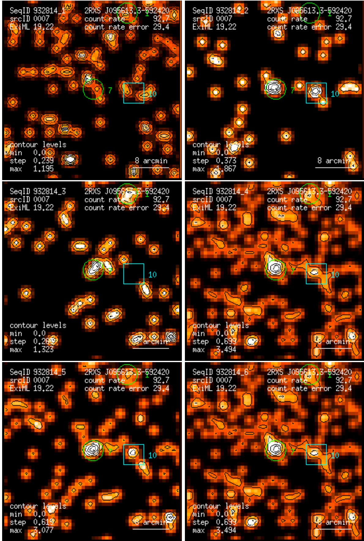
Figure 7: RASS 932814: detection 0007: band rate images, Gaussian filter: (1) PSPC channels 11 – 41, (2) 52 – 90, (3) 91 – 201, (4) 11 – 235, (5) 52 – 201, (6) 11 – 201. Broad band rates in counts/ks. Band rate contour levels in counts/ks/arcmin 2 .
