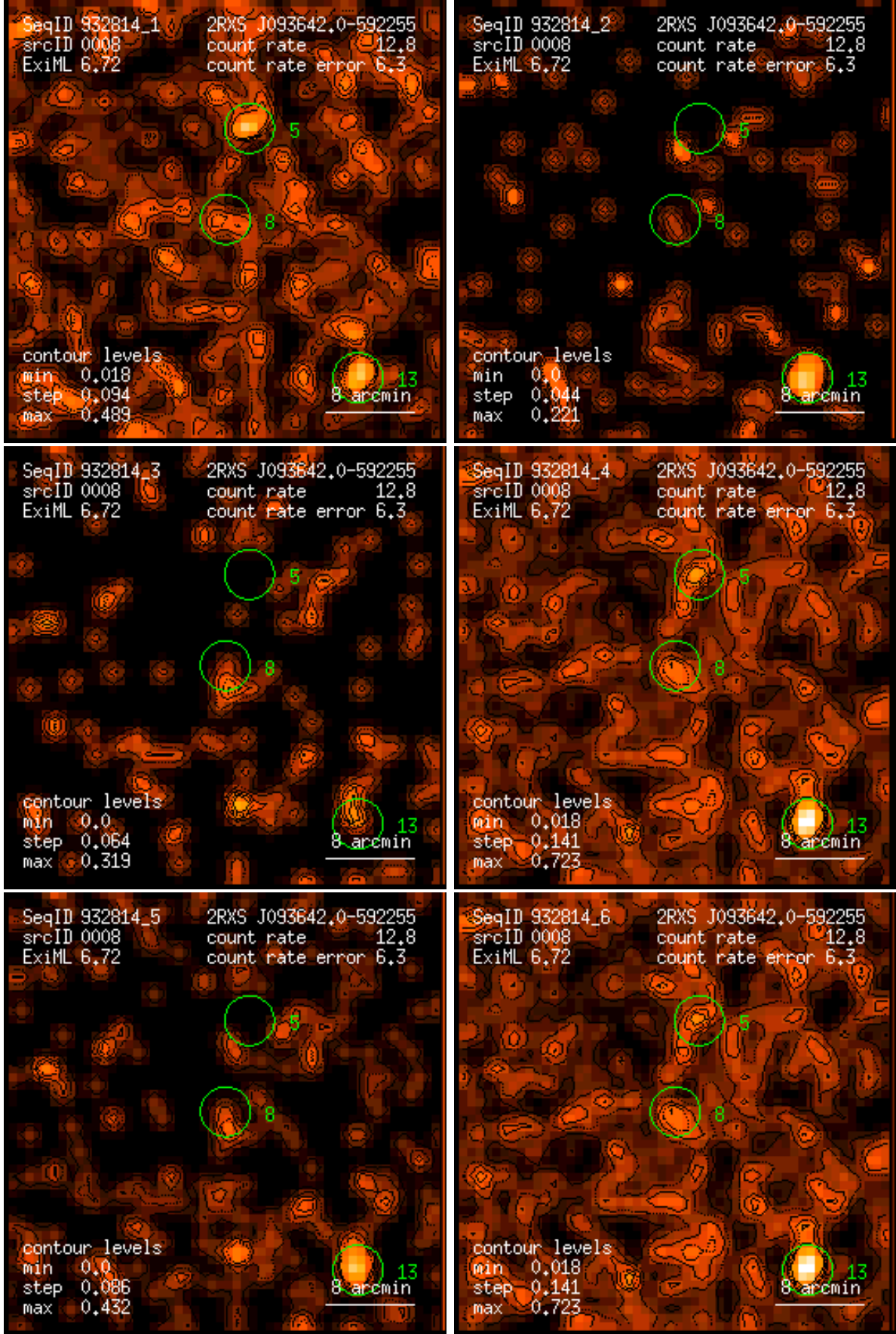
Figure 8: RASS 932814: detection 0008: band rate images, Gaussian filter: (1) PSPC channels 11 – 41, (2) 52 – 90, (3) 91 – 201, (4) 11 – 235, (5) 52 – 201, (6) 11 – 201. Broad band rates in counts/ks. Band rate contour levels in counts/ks/arcmin 2 .
