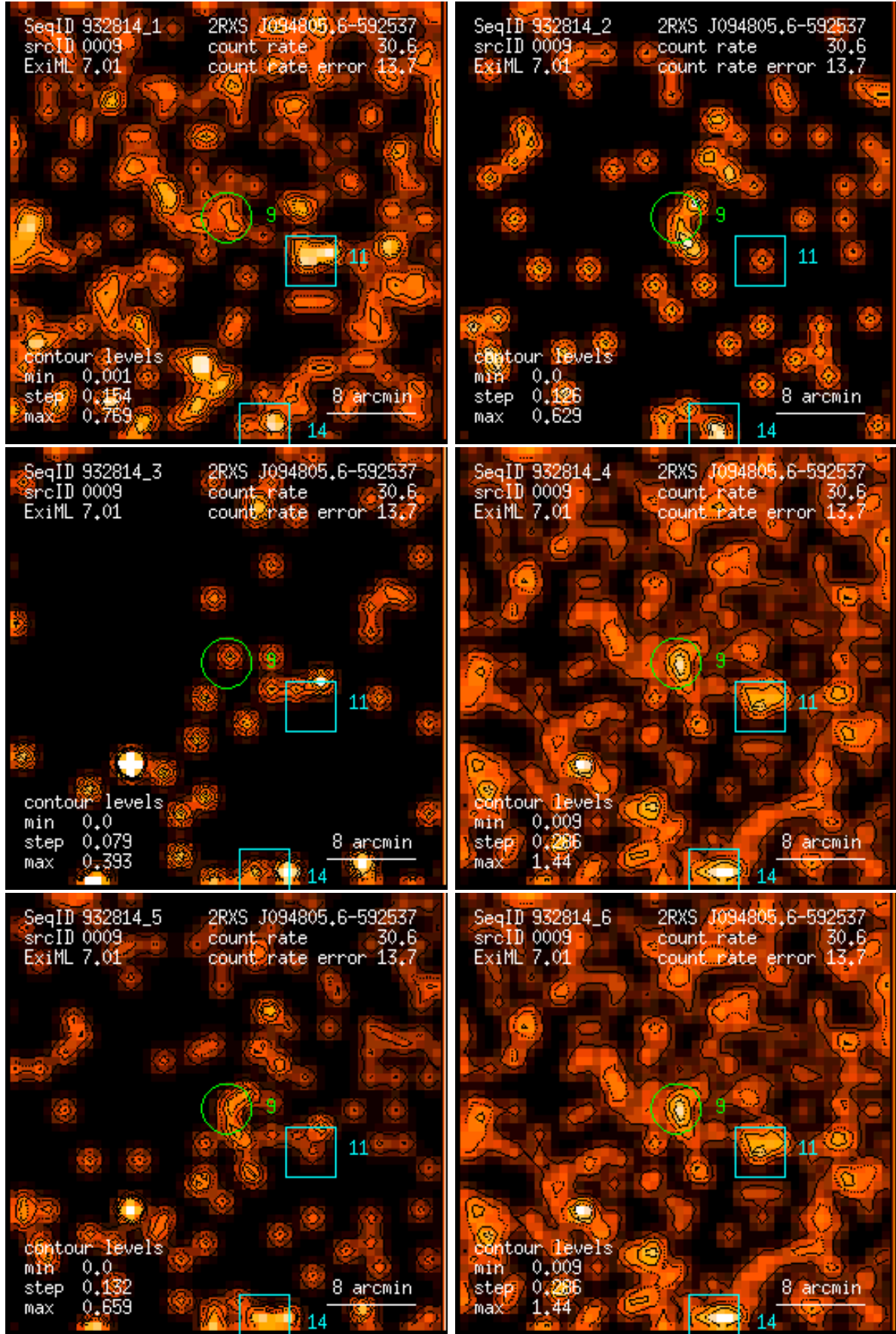
Figure 9: RASS 932814: detection 0009: band rate images, Gaussian filter: (1) PSPC channels 11 – 41, (2) 52 – 90, (3) 91 – 201, (4) 11 – 235, (5) 52 – 201, (6) 11 – 201. Broad band rates in counts/ks. Band rate contour levels in counts/ks/arcmin 2 .
